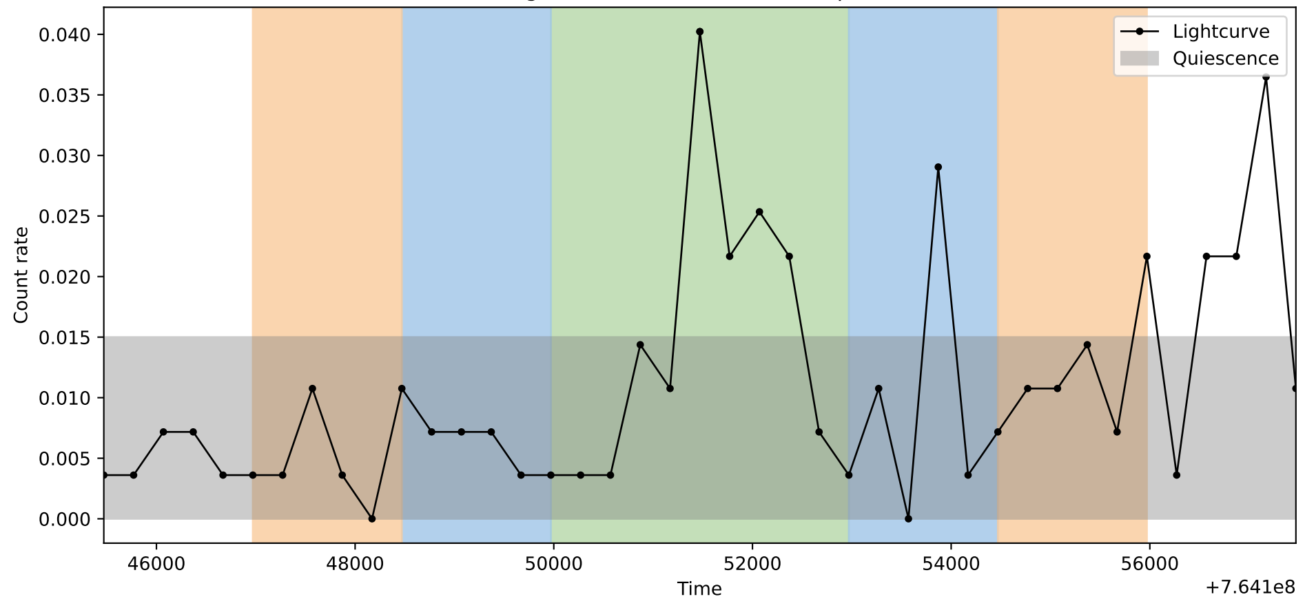
Lightcurve ObsID: 25297, Shape: 2
