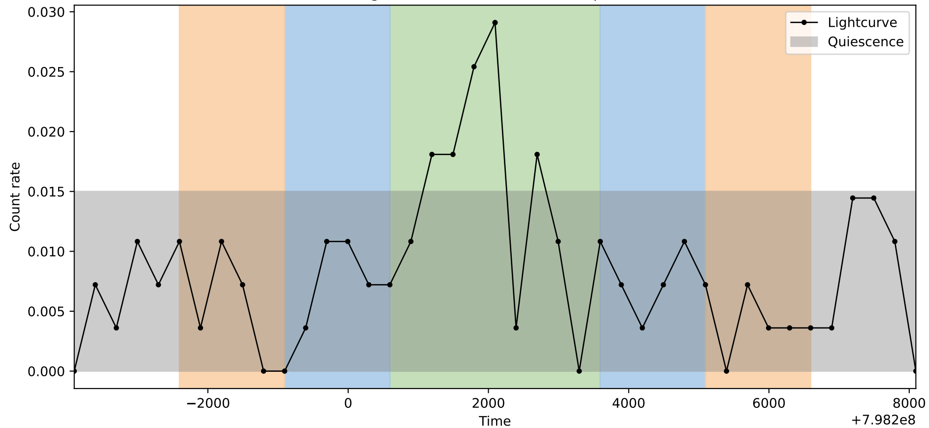
Lightcurve ObsID: 26759, Shape: 1
