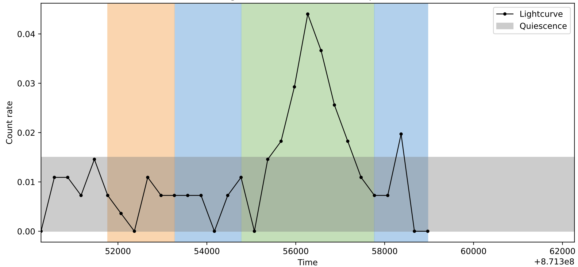
Lightcurve ObsID: 31022, Shape: 1
