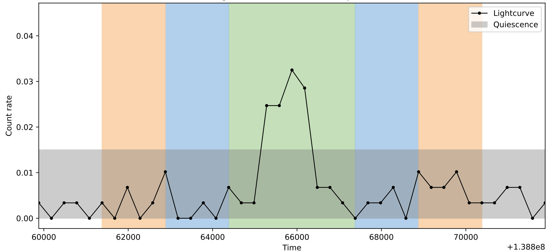
Lightcurve ObsID: 3392, Shape: 1
