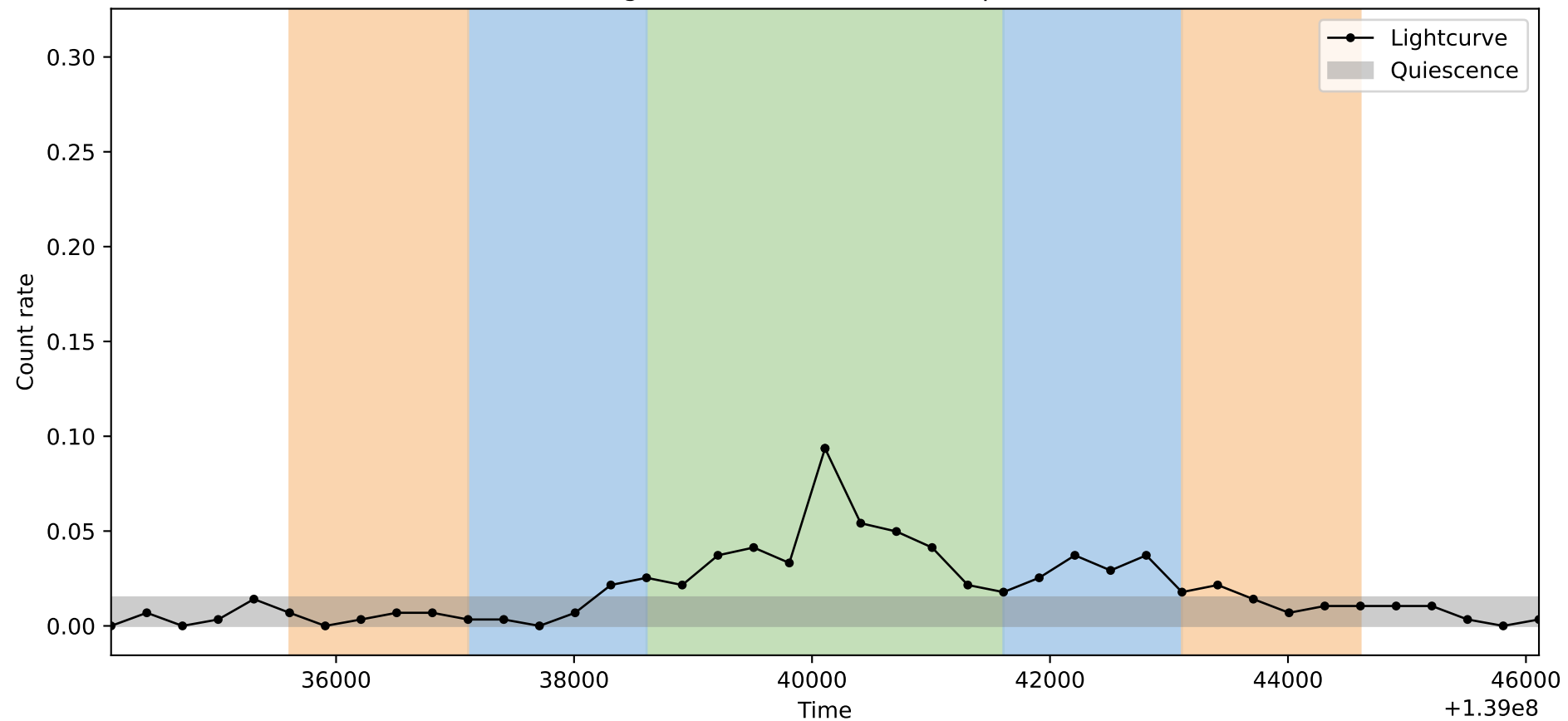
Lightcurve ObsID: 3393, Shape: 2
