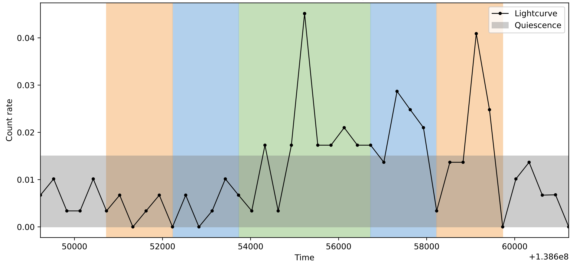
Lightcurve ObsID: 3663, Shape: 2
