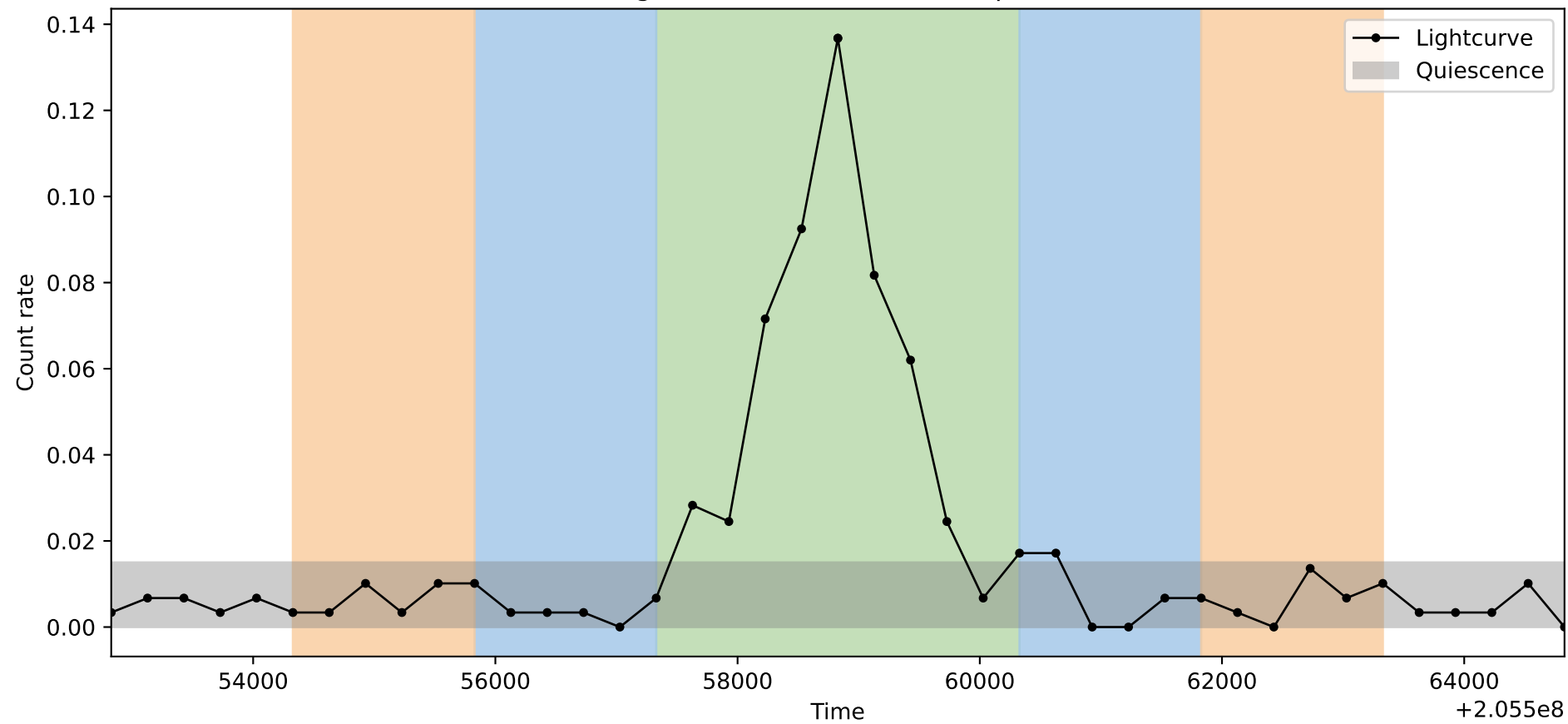
Lightcurve ObsID: 4684, Shape: 1
