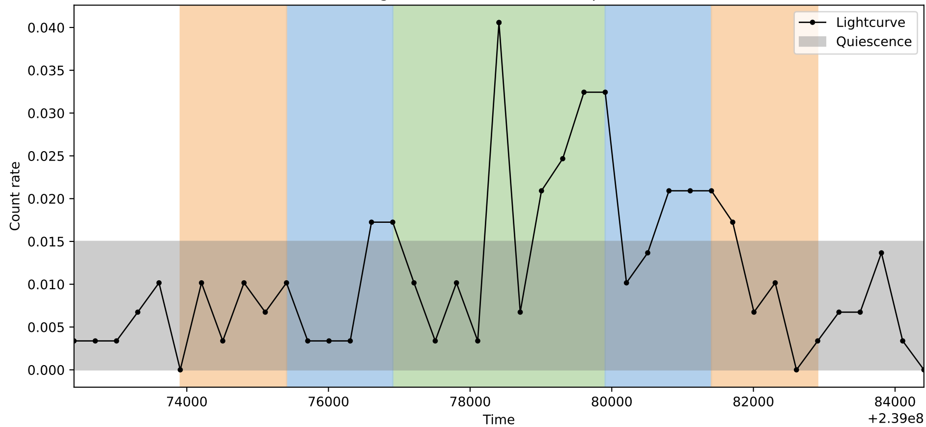
Lightcurve ObsID: 5952, Shape: 2
