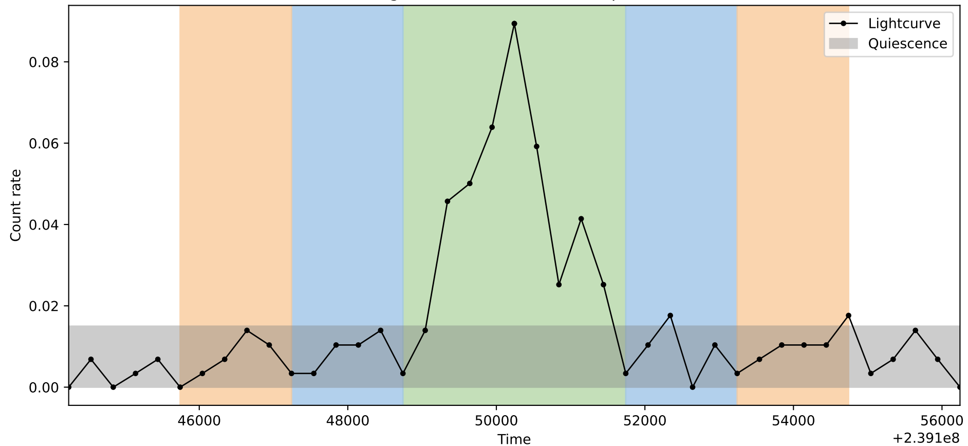
Lightcurve ObsID: 5953, Shape: 2
