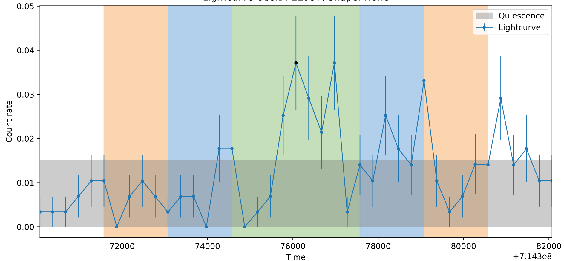
Lightcurve ObsID: 22937, Shape: None
