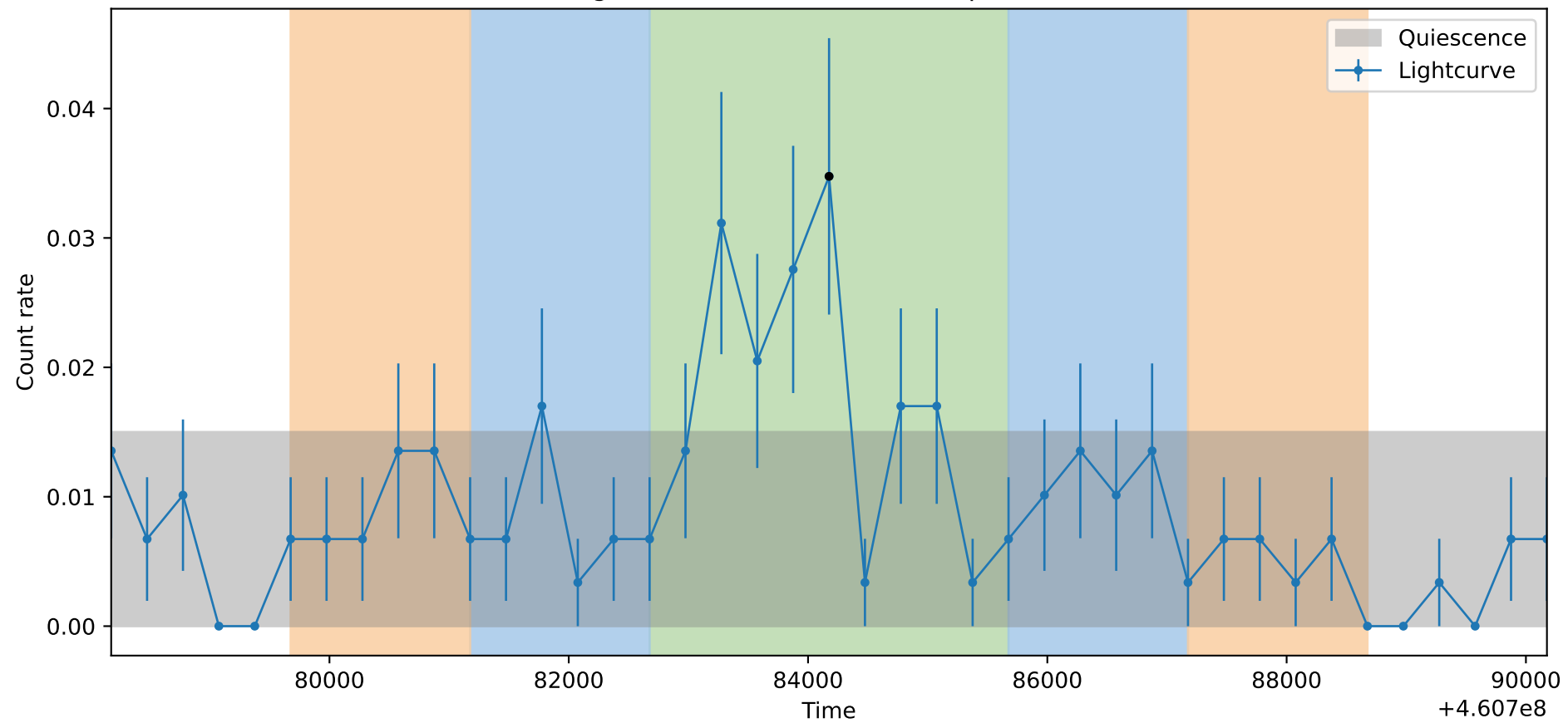
Lightcurve ObsID: 14439, Shape: None
