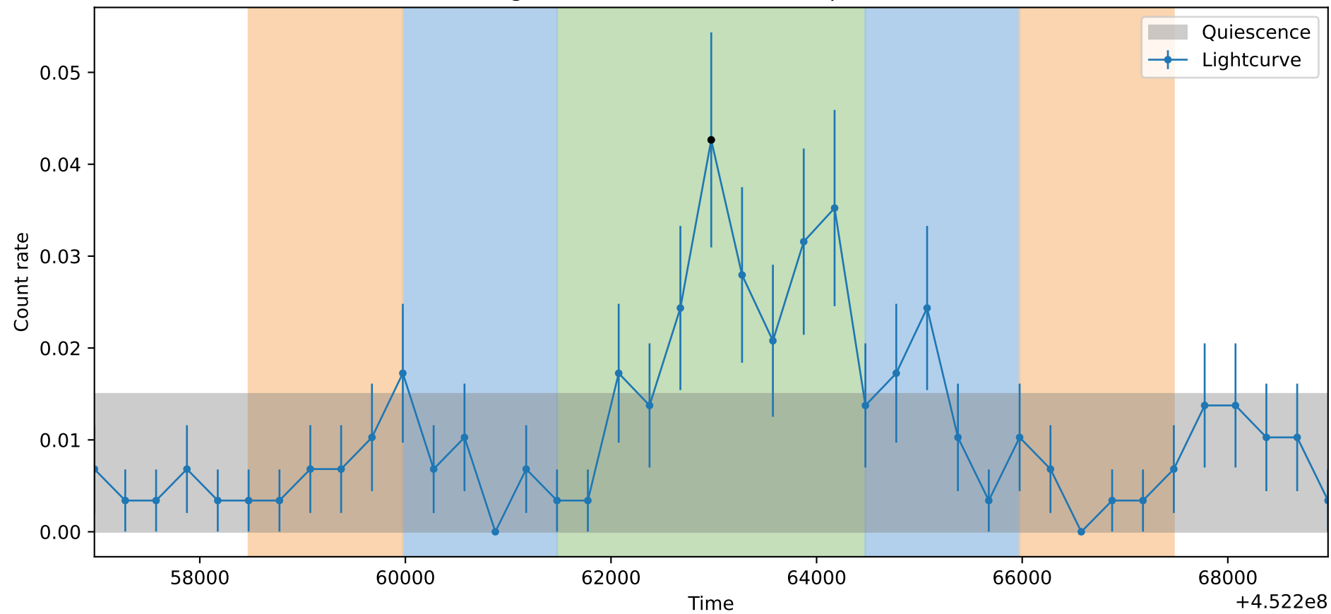
Lightcurve ObsID: 13847, Shape: None
