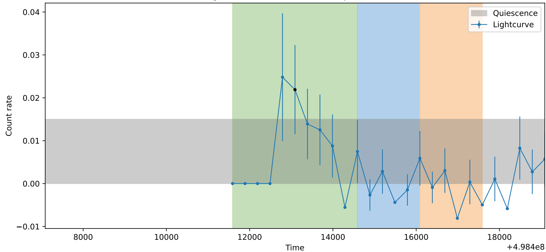
Lightcurve ObsID: 14943, Shape: None
