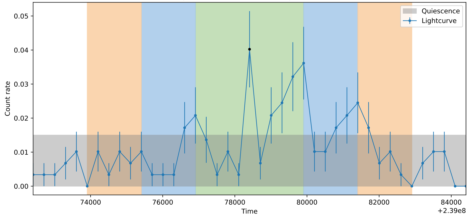
Lightcurve ObsID: 5952, Shape: None
