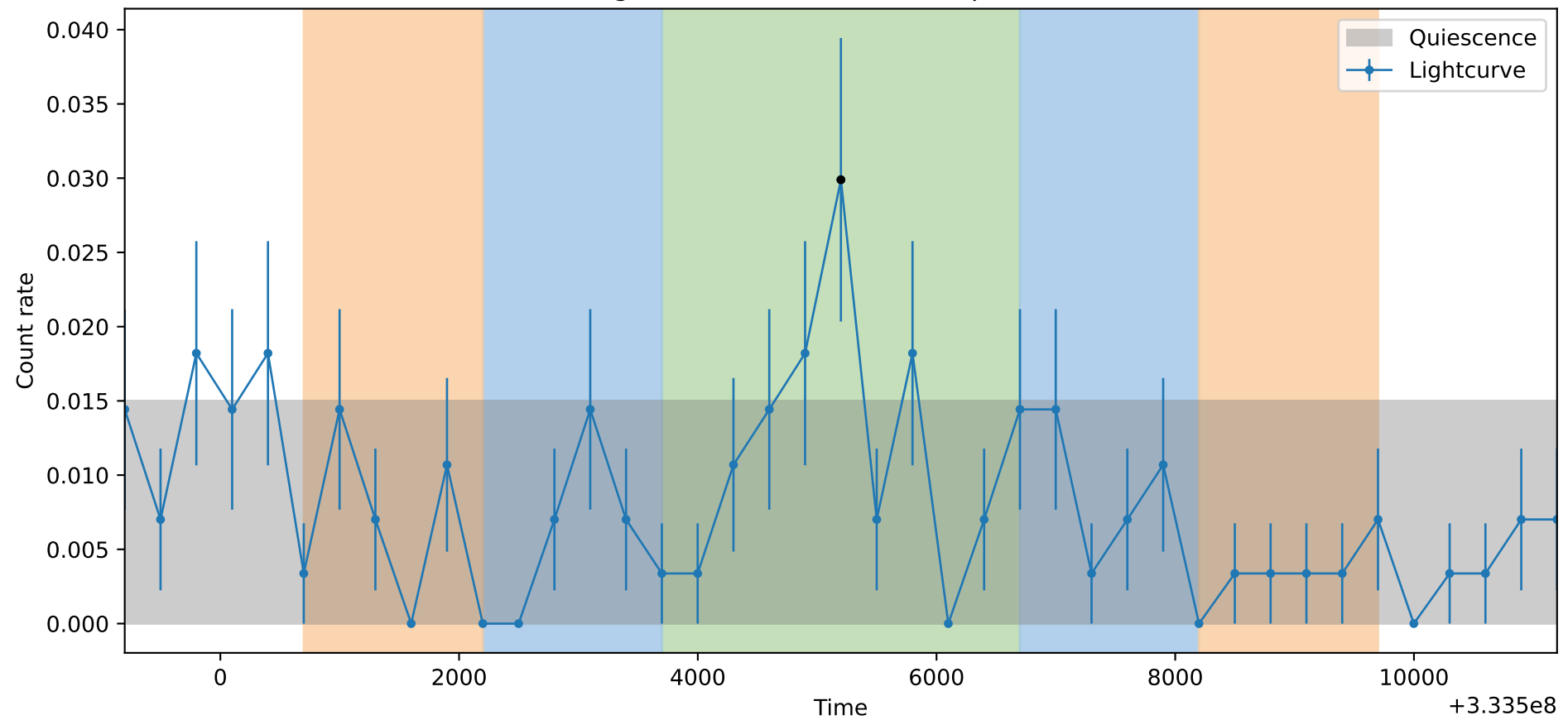
Lightcurve ObsID: 9173, Shape: None
