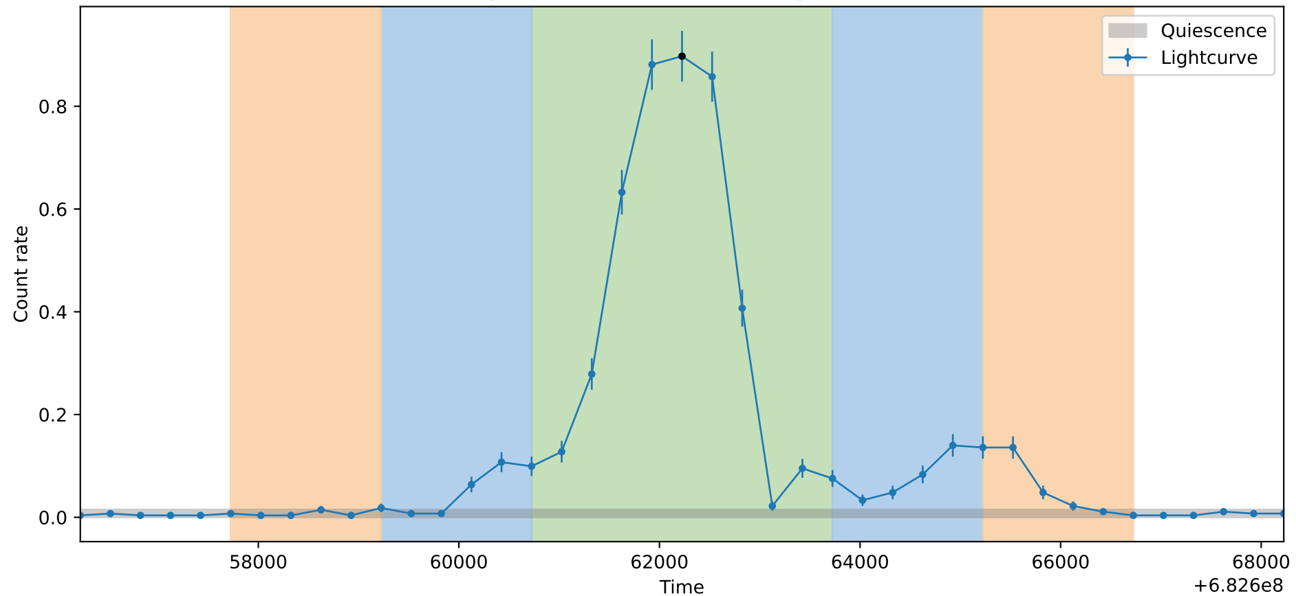
Lightcurve ObsID: 20751, Shape: None
