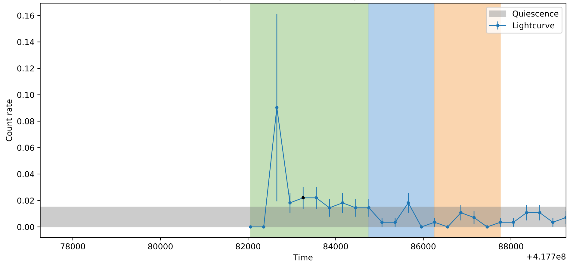
Lightcurve ObsID: 13016, Shape: None
