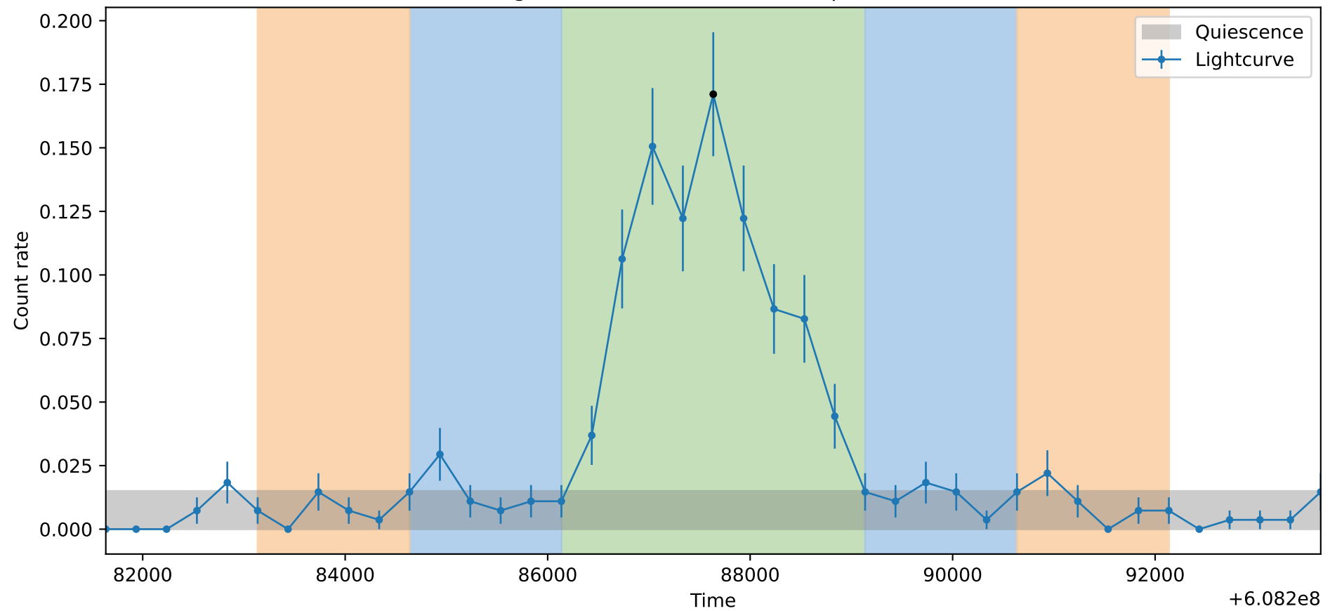
Lightcurve ObsID: 20041, Shape: None
