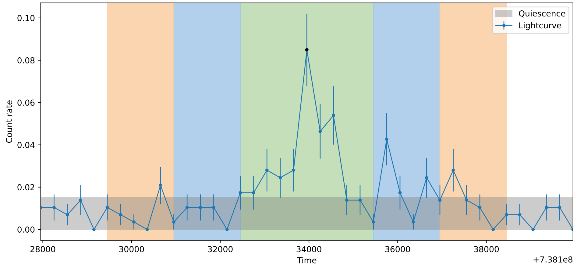
Lightcurve ObsID: 22592, Shape: None
