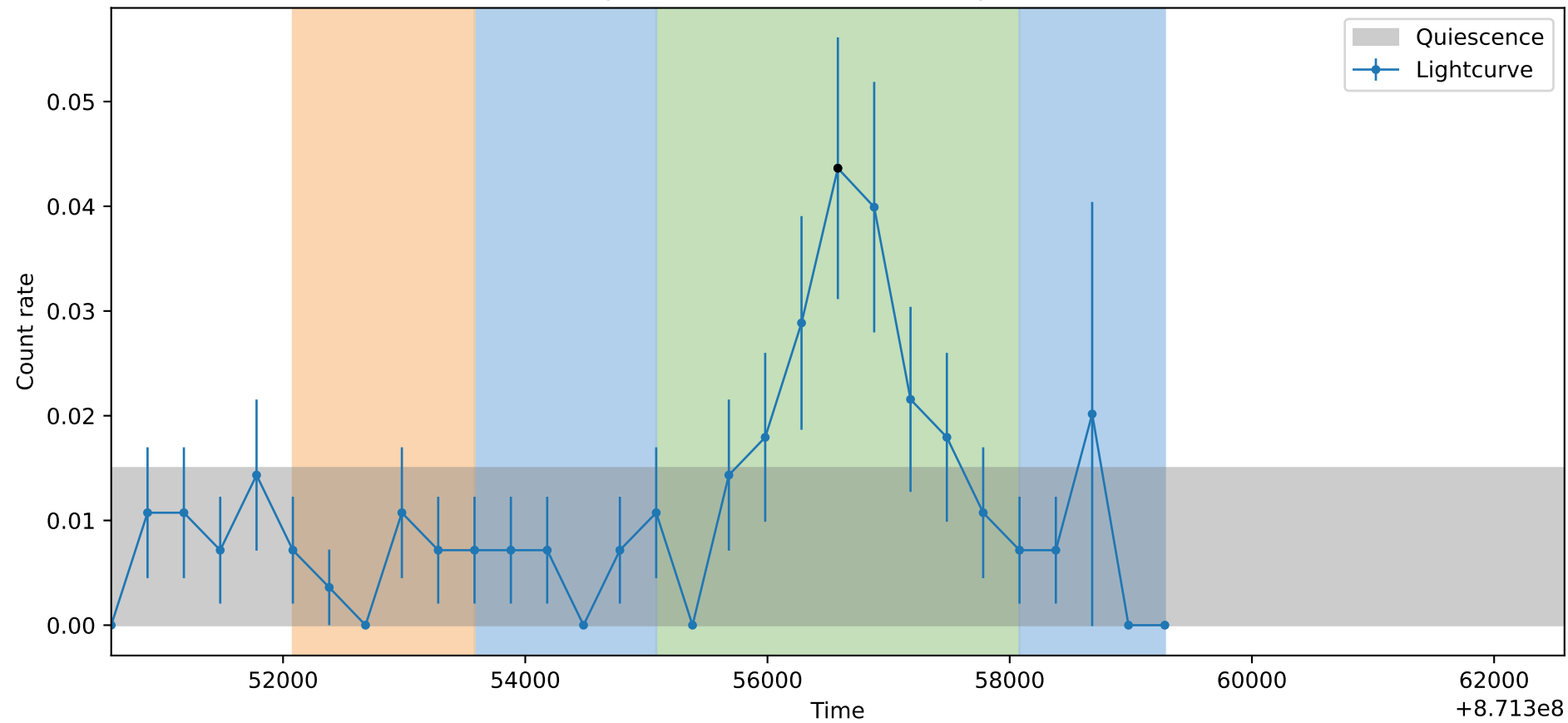
Lightcurve ObsID: 31022, Shape: None
