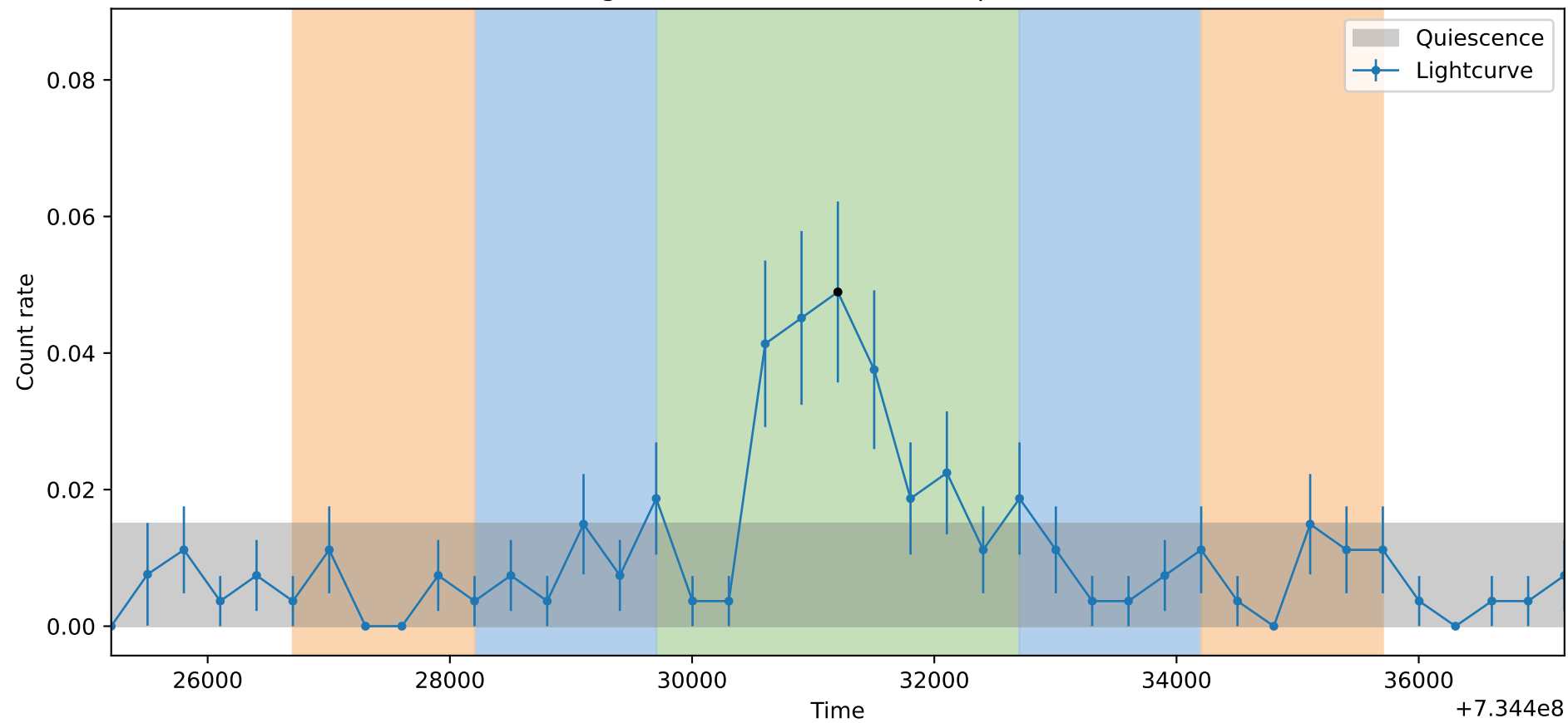
Lightcurve ObsID: 23665, Shape: None
