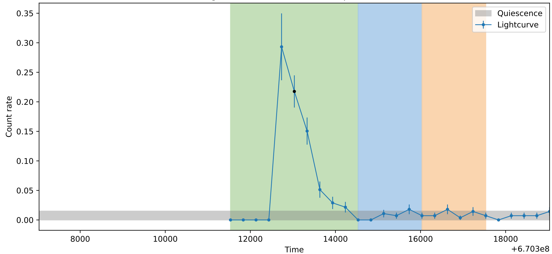
Lightcurve ObsID: 21454, Shape: None
