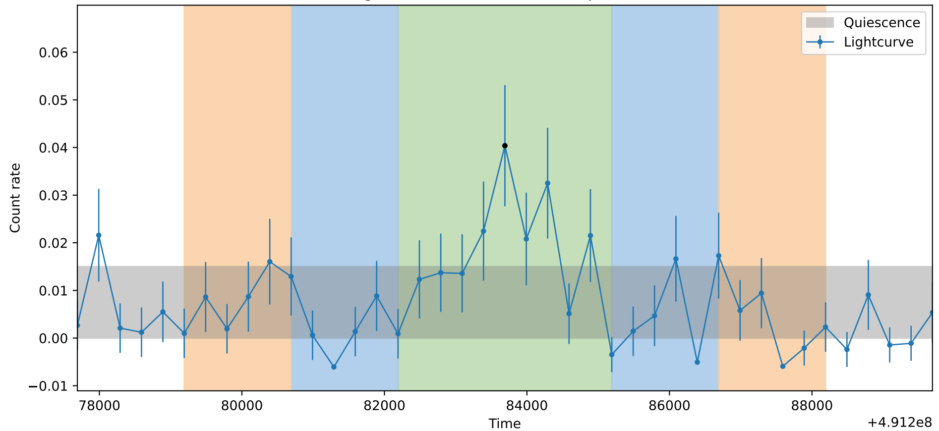
Lightcurve ObsID: 15041, Shape: None
