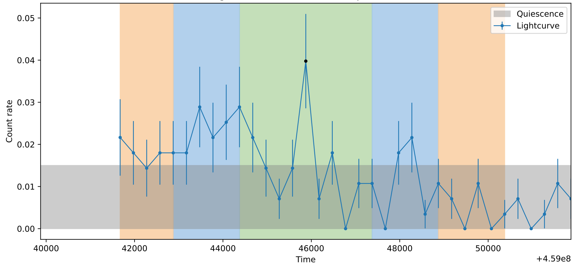
Lightcurve ObsID: 14465, Shape: None
