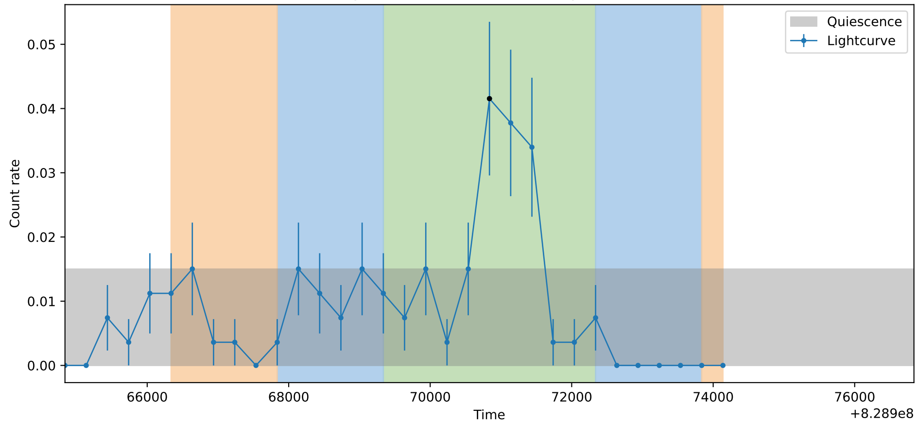
Lightcurve ObsID: 28231, Shape: None
