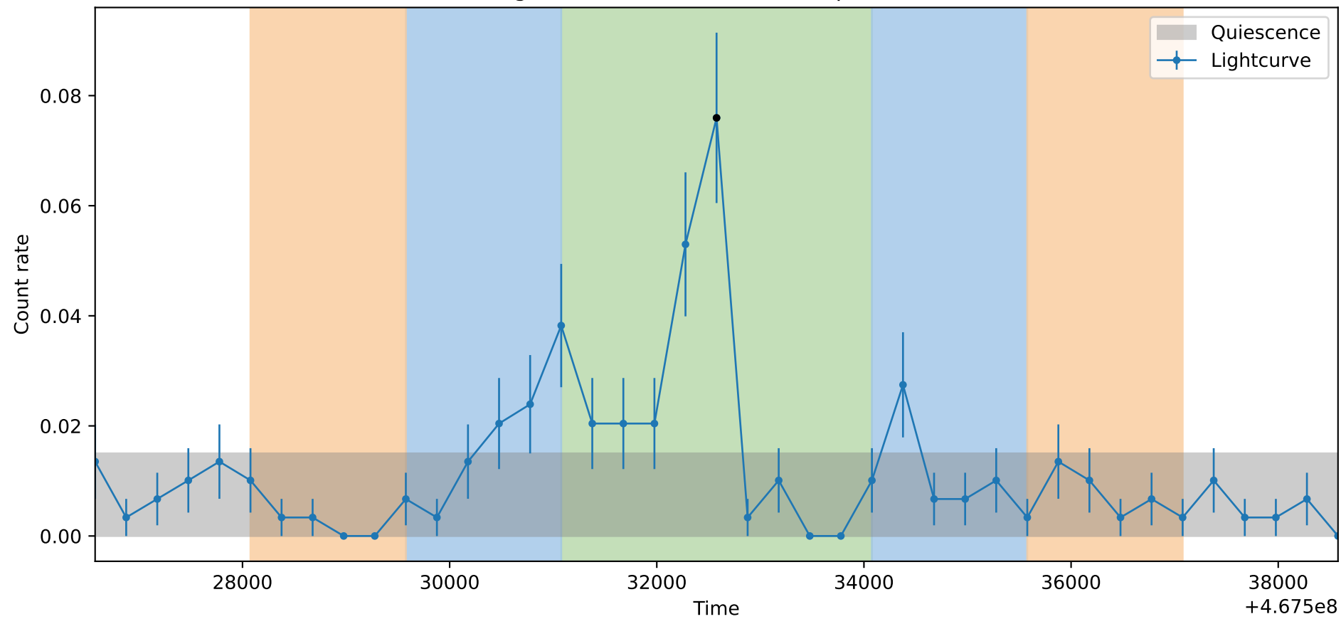
Lightcurve ObsID: 15570, Shape: None
