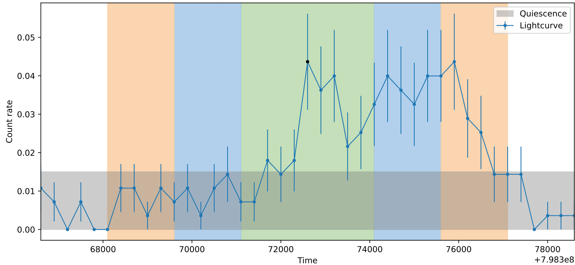
Lightcurve ObsID: 26760, Shape: None
