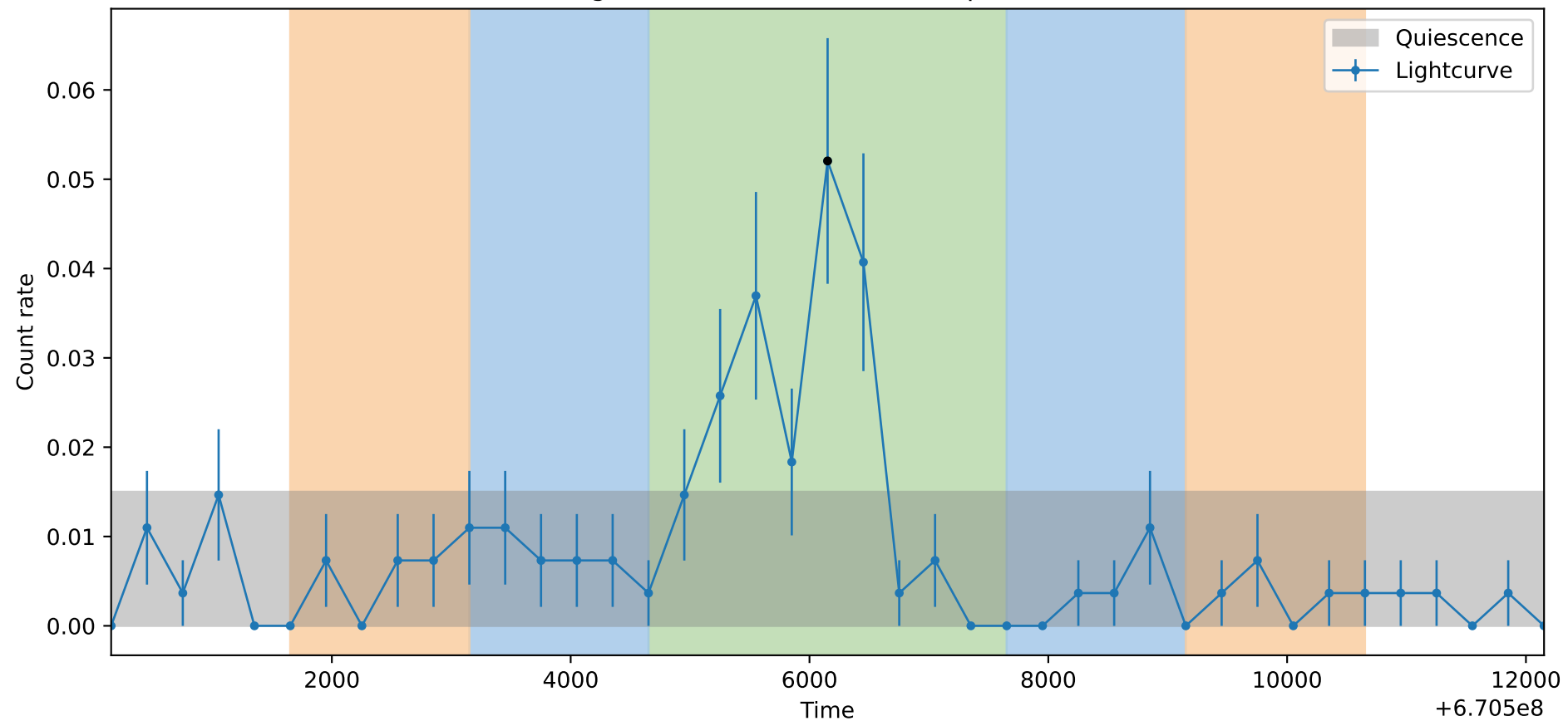
Lightcurve ObsID: 21456, Shape: None
