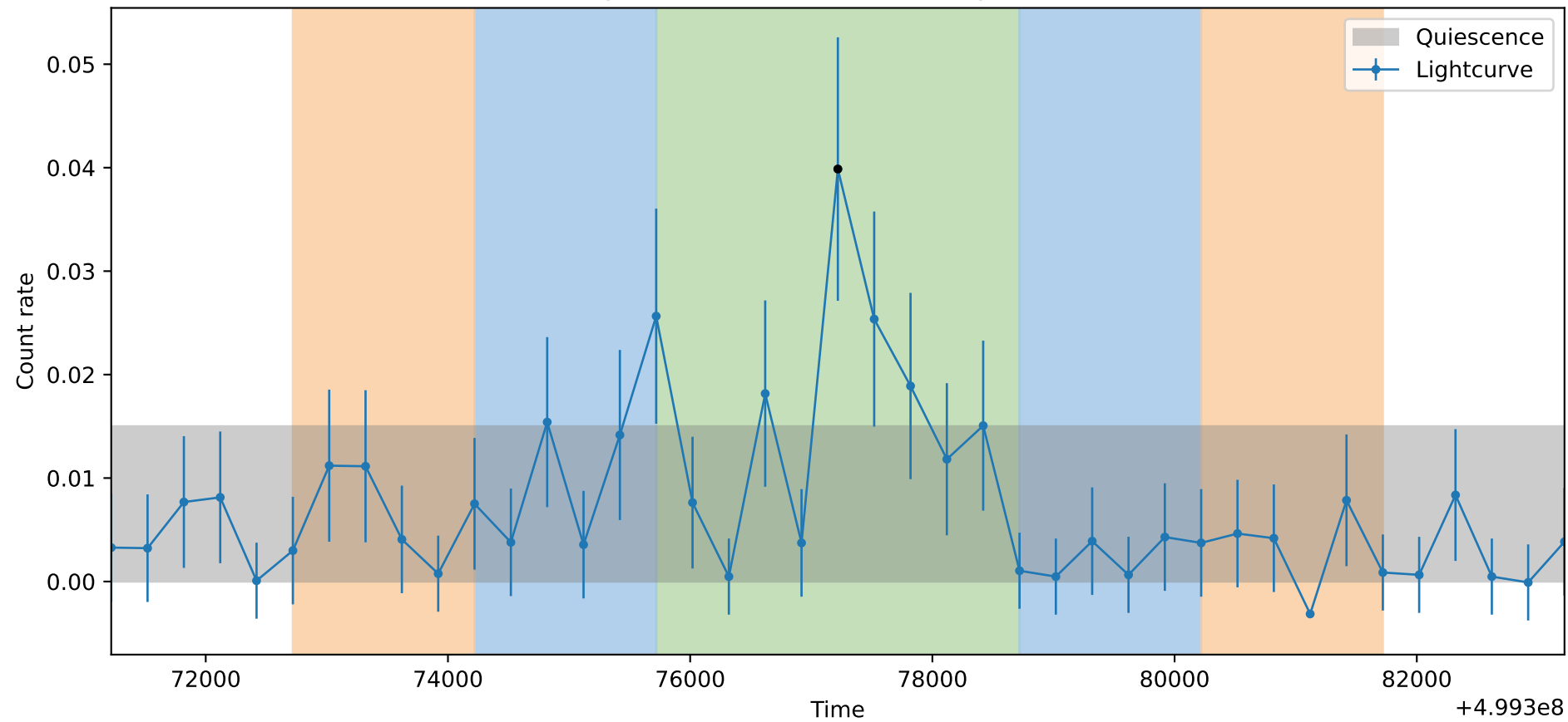
Lightcurve ObsID: 15045, Shape: None
