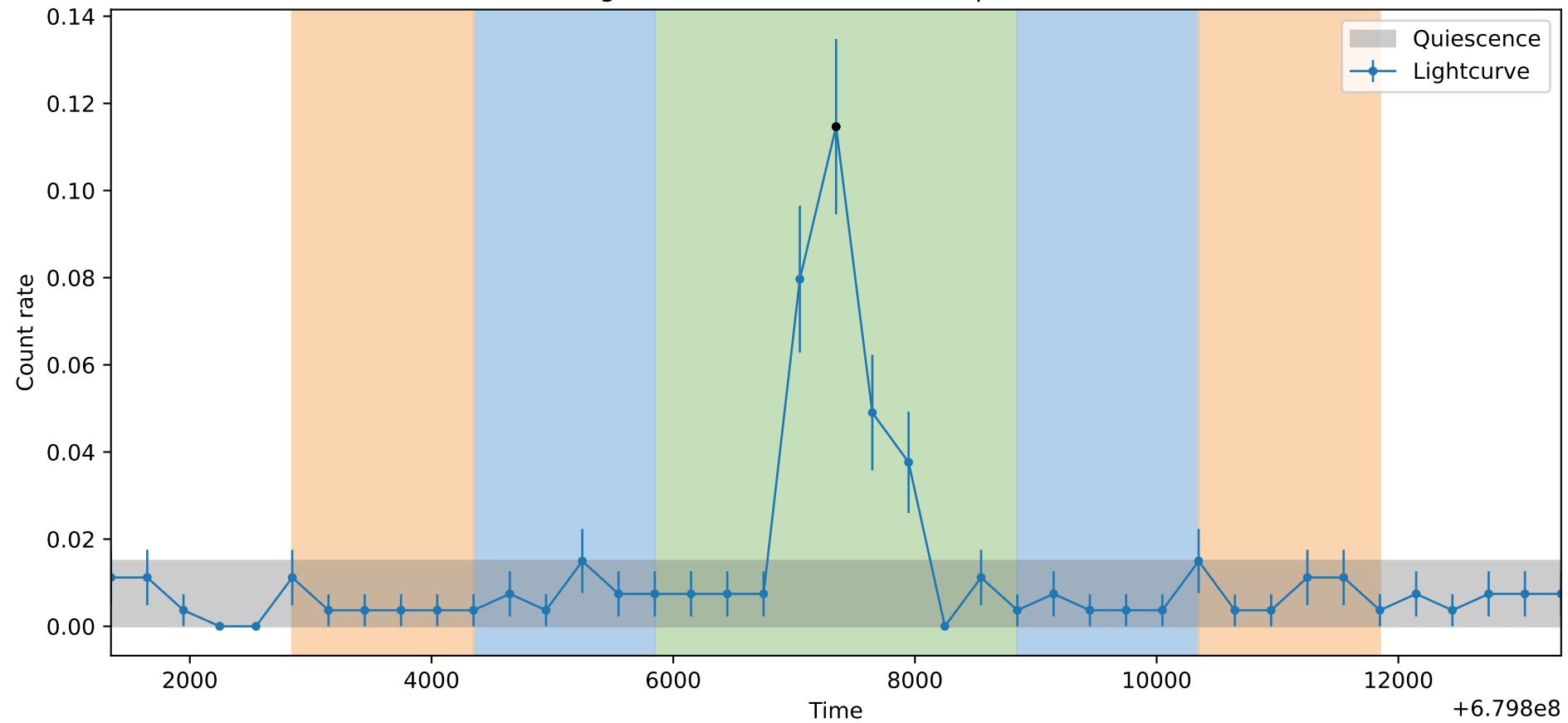
Lightcurve ObsID: 22230, Shape: None
