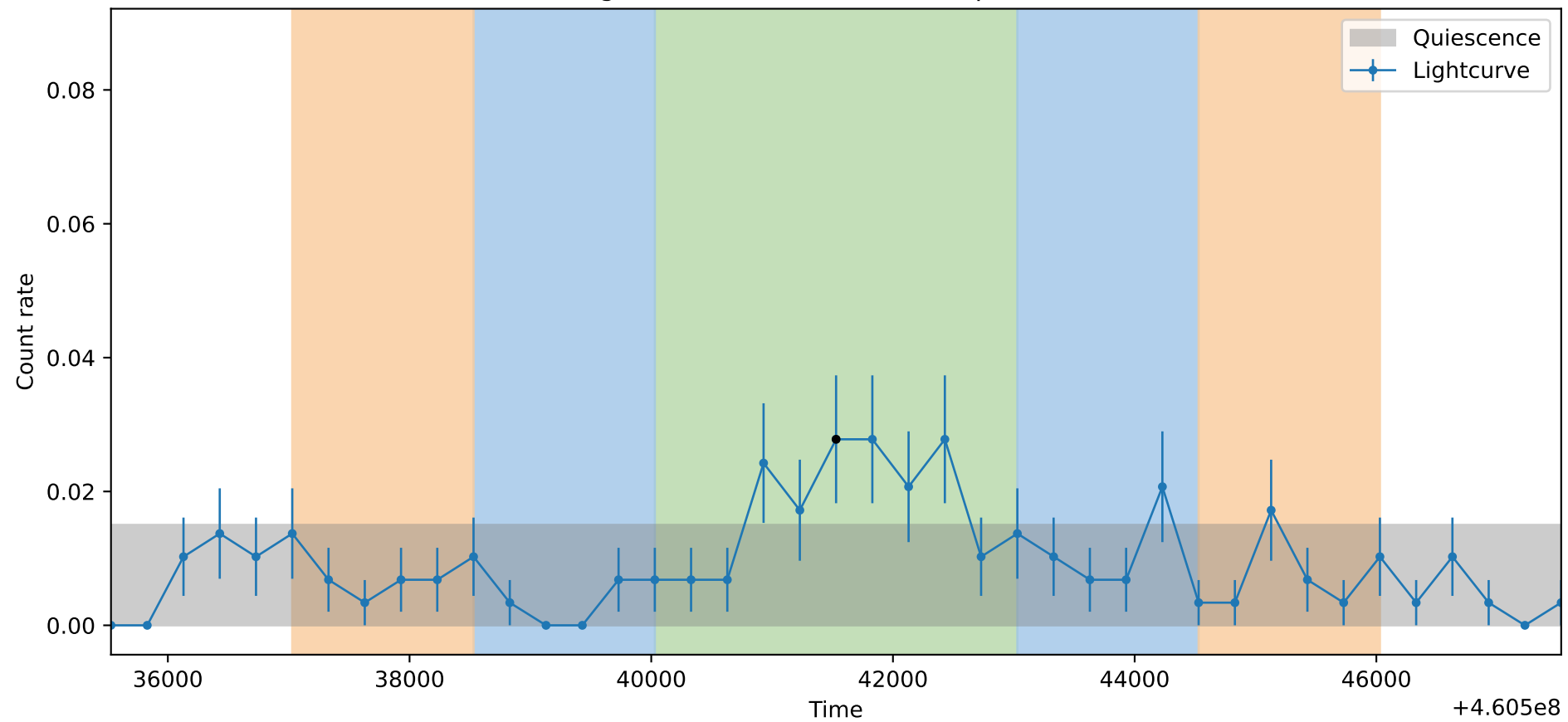
Lightcurve ObsID: 13852, Shape: None
