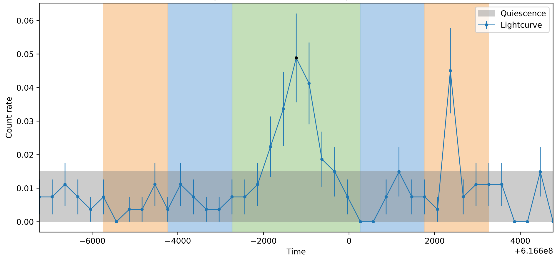
Lightcurve ObsID: 19703, Shape: None
