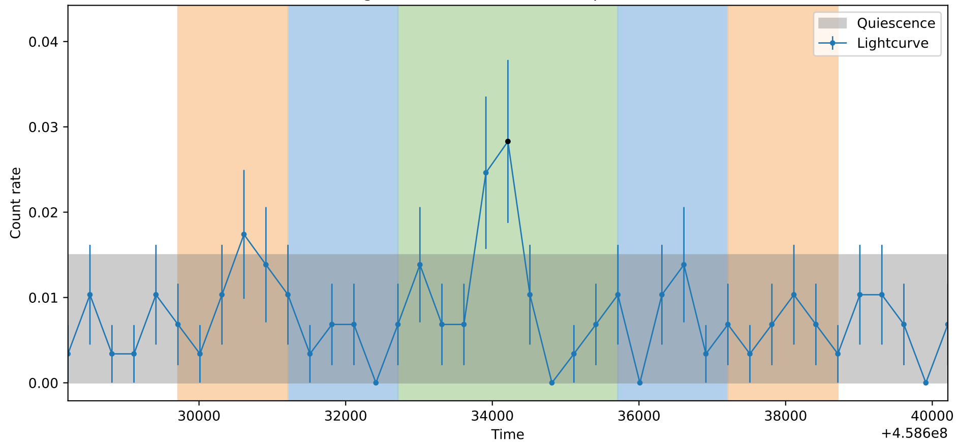
Lightcurve ObsID: 13853, Shape: None
