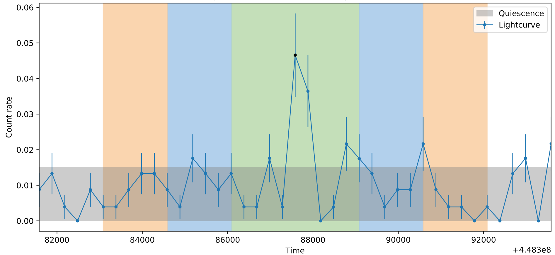
Lightcurve ObsID: 13857, Shape: None
