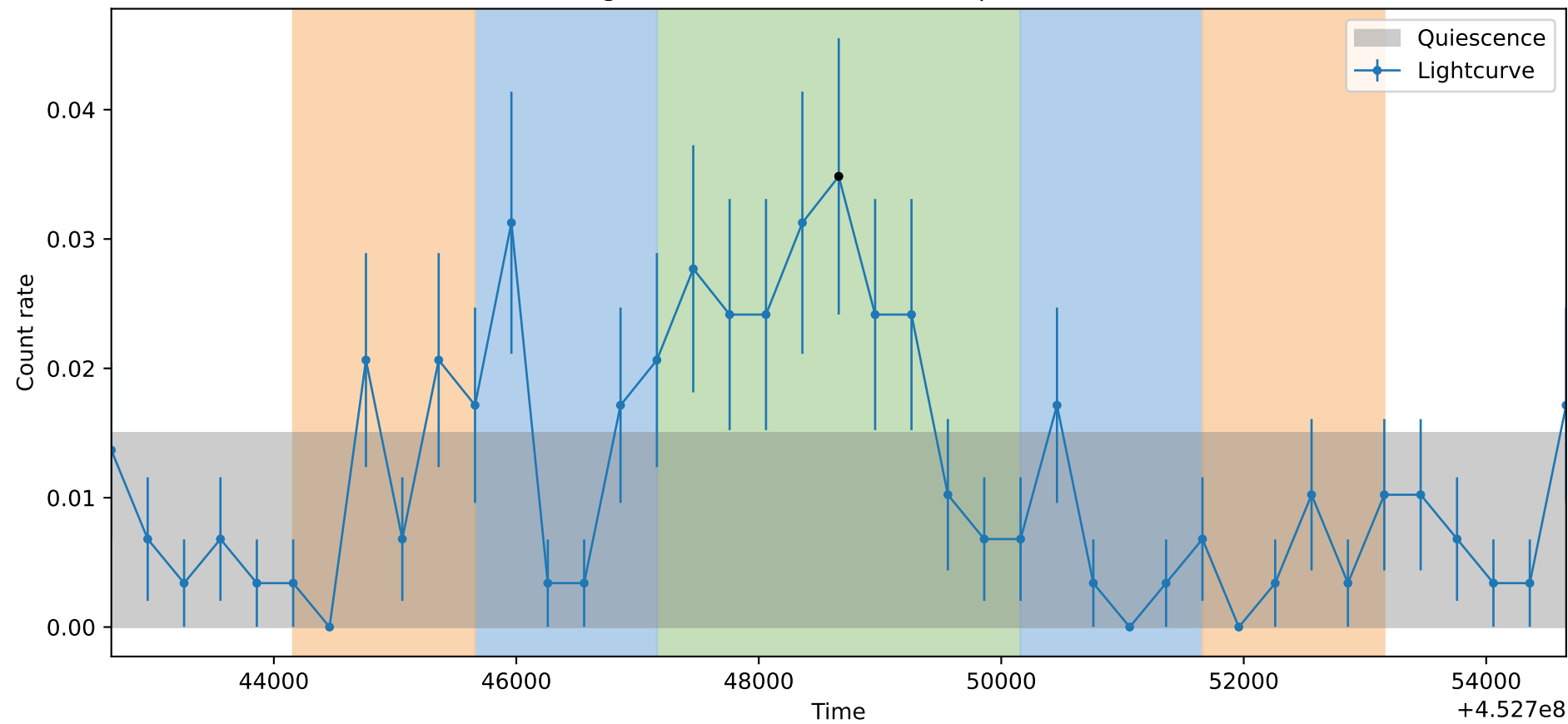
Lightcurve ObsID: 14427, Shape: None
