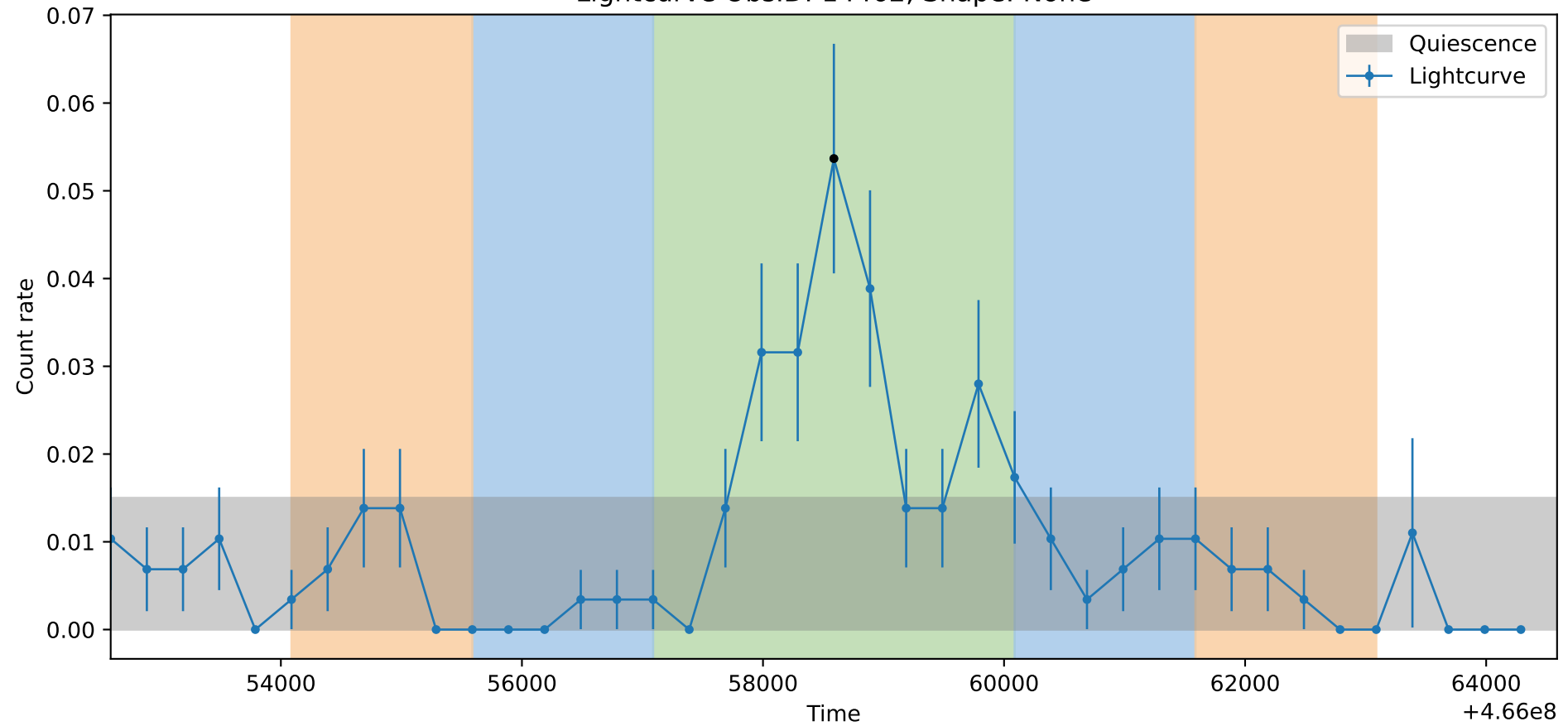
Lightcurve ObsID: 14462, Shape: None
