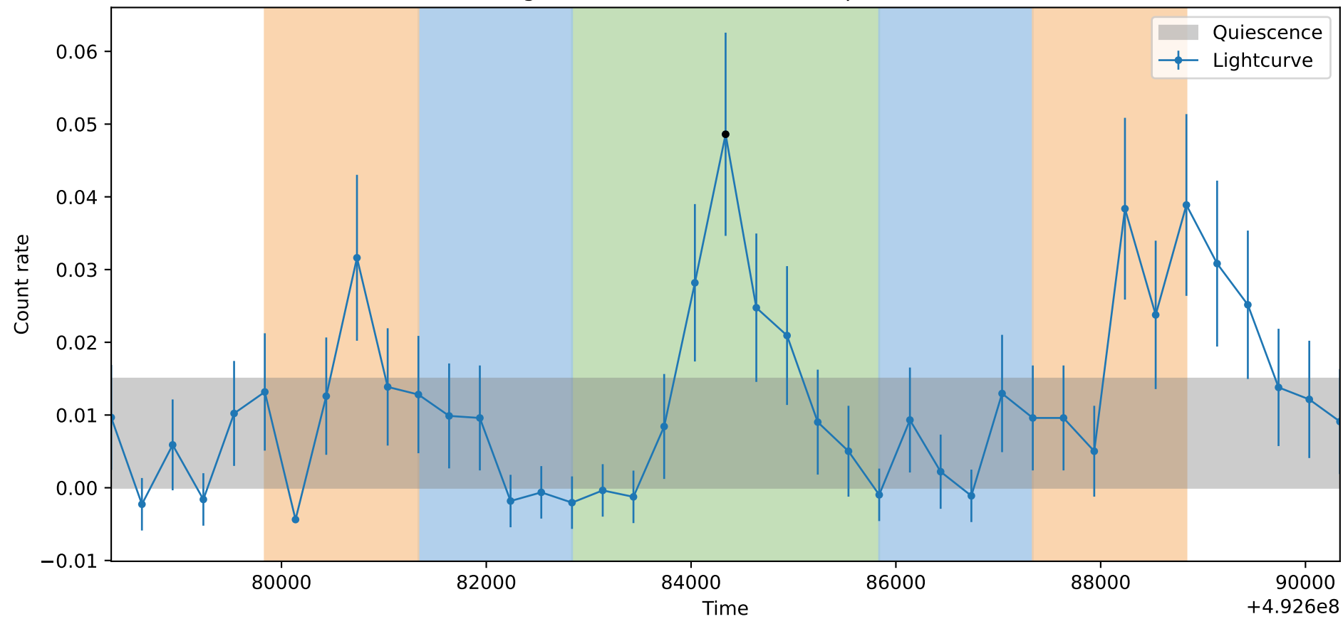
Lightcurve ObsID: 15042, Shape: None
