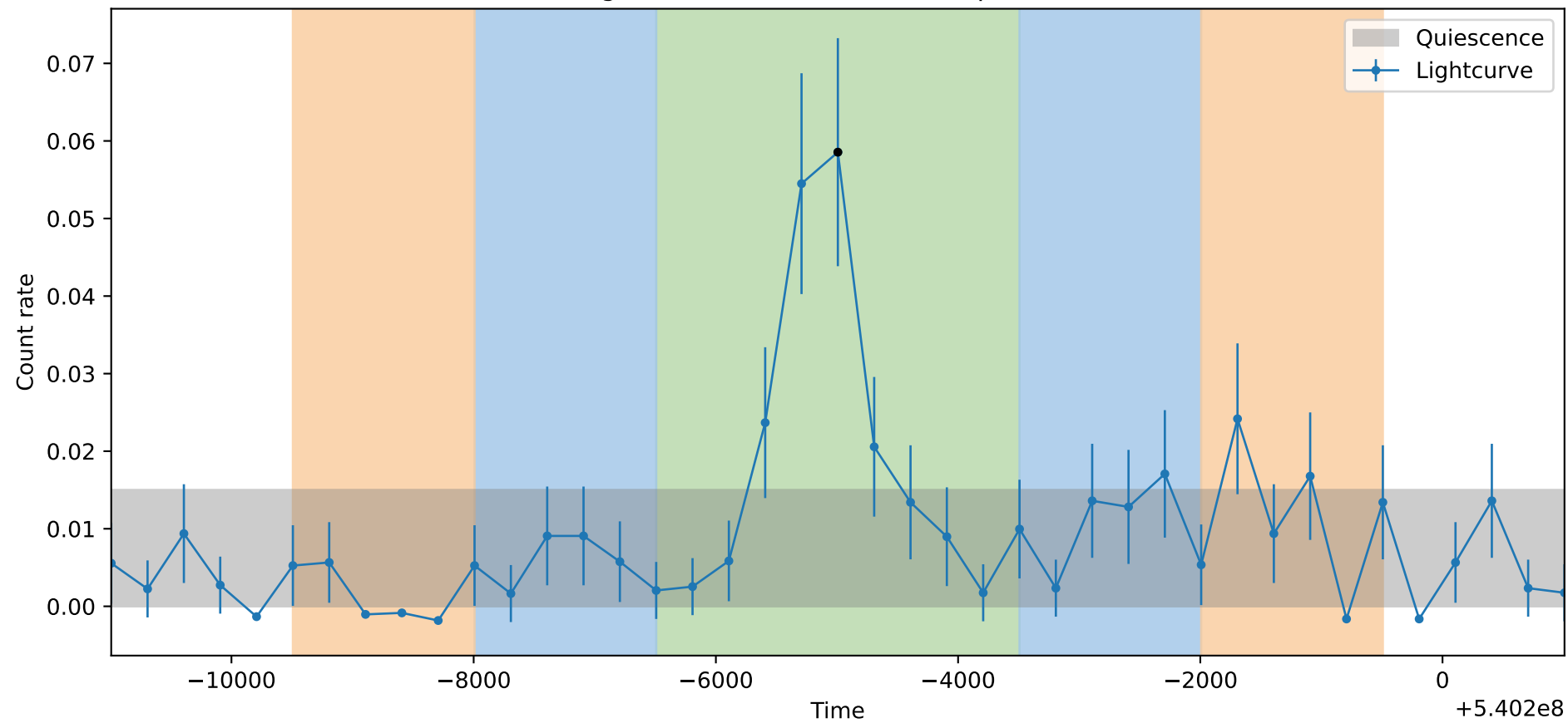
Lightcurve ObsID: 16963, Shape: None
