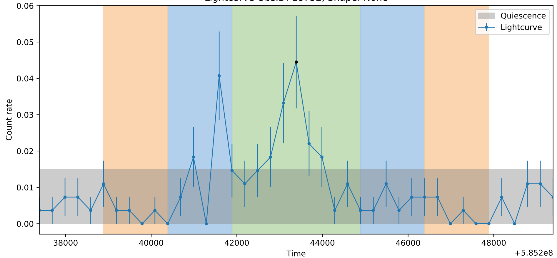
Lightcurve ObsID: 18732, Shape: None
