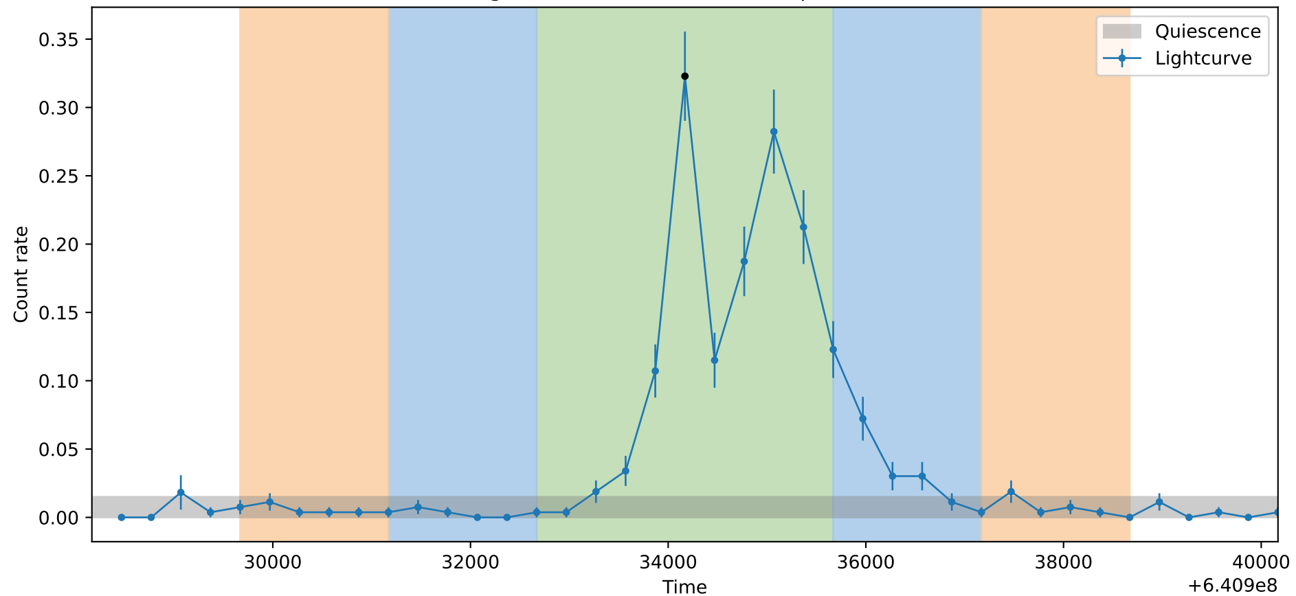
Lightcurve ObsID: 20346, Shape: None
