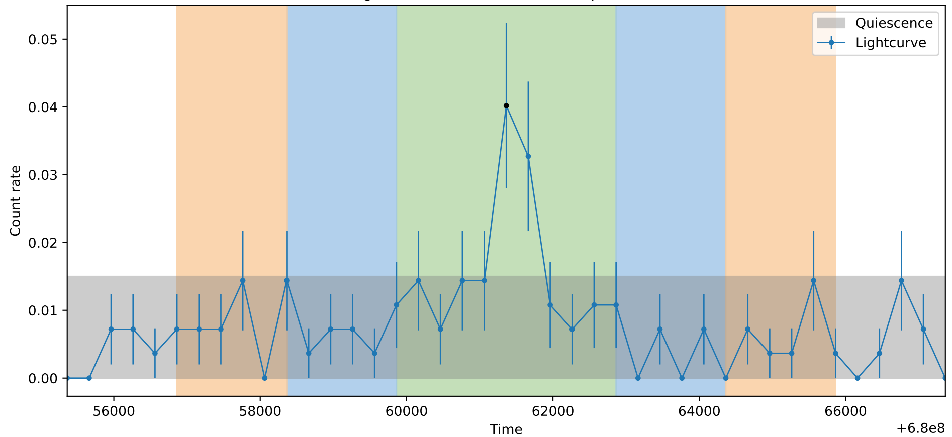
Lightcurve ObsID: 20446, Shape: None
