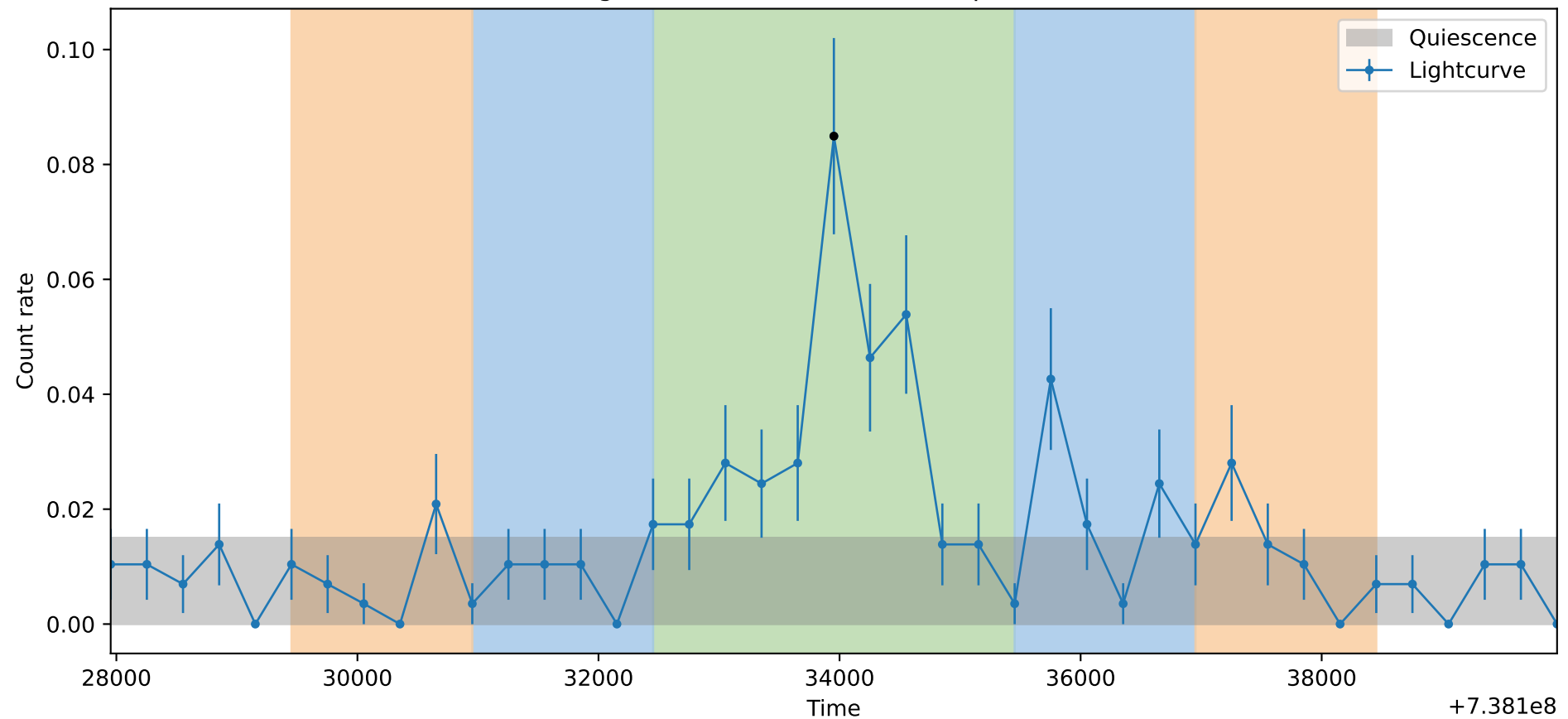
Lightcurve ObsID: 22592, Shape: None
