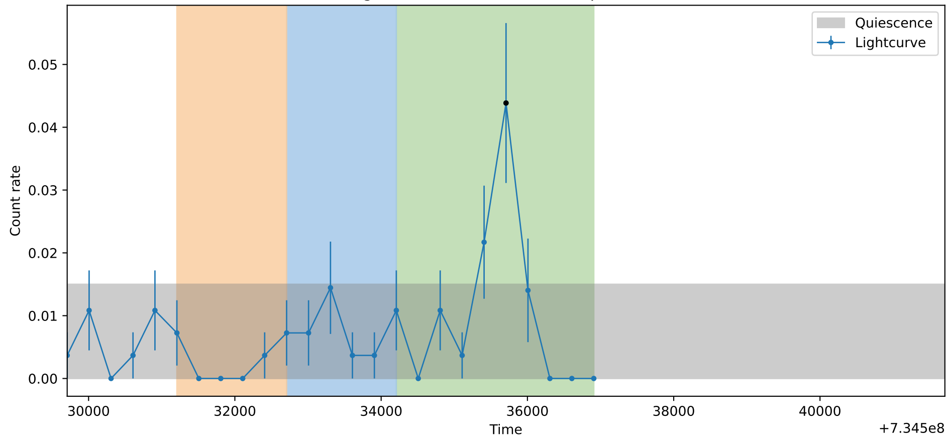
Lightcurve ObsID: 23666, Shape: None
