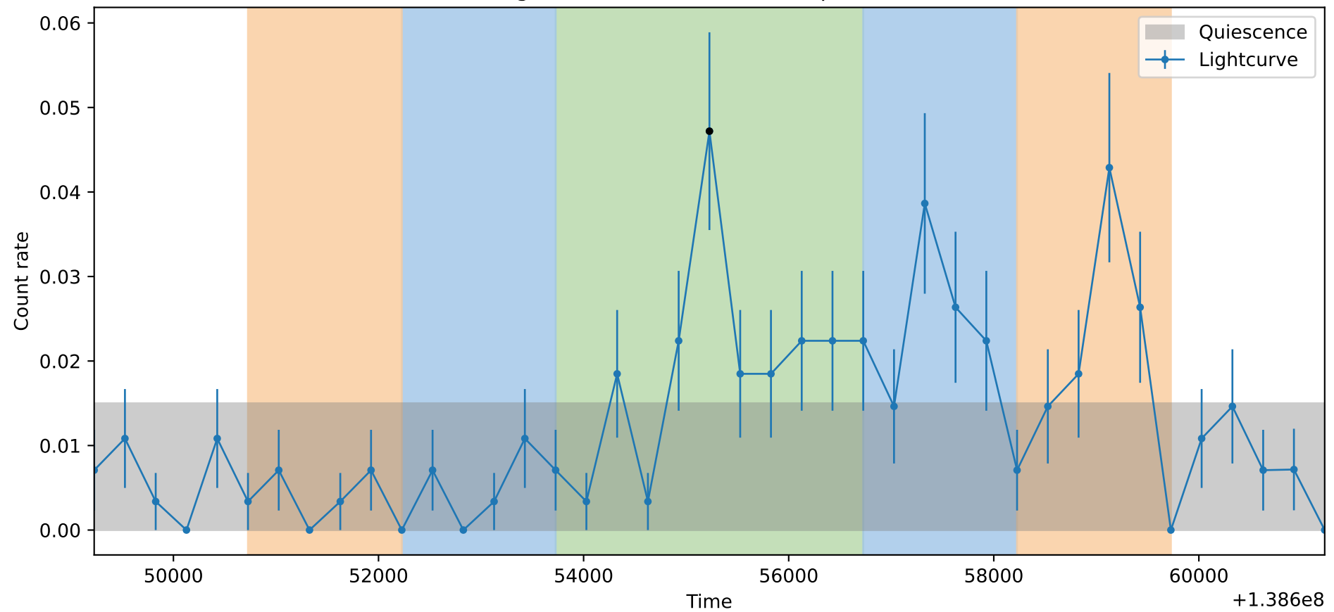
Lightcurve ObsID: 3663, Shape: None
