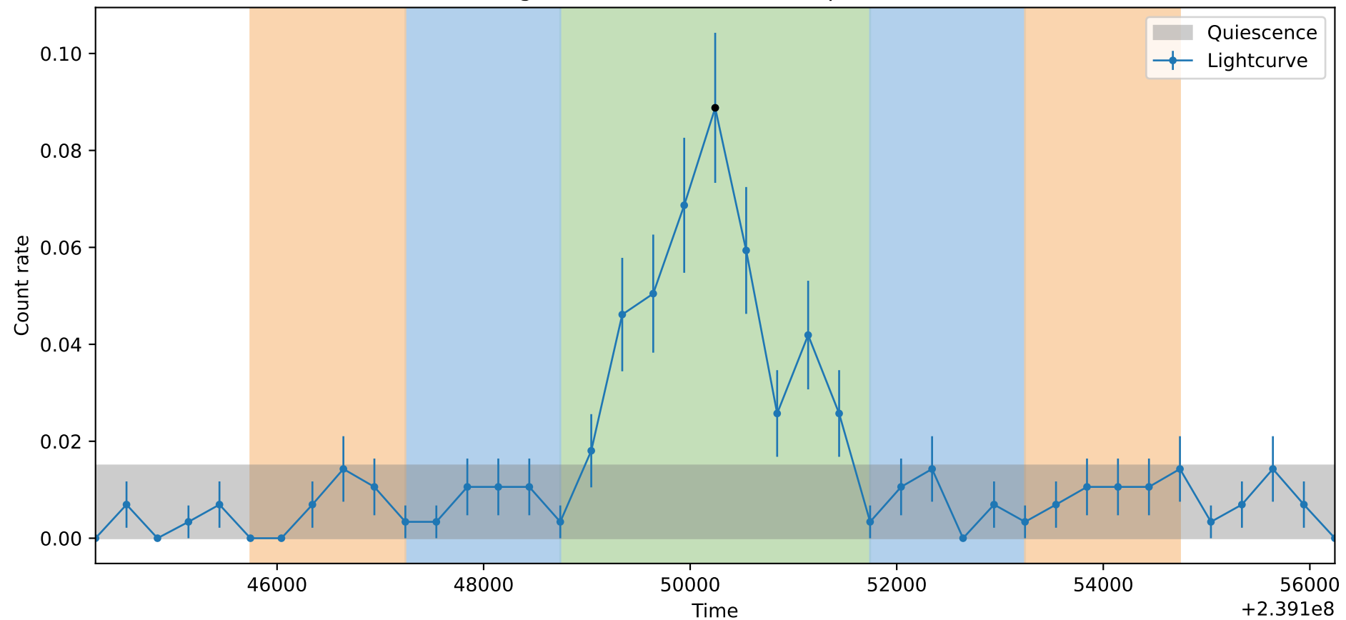
Lightcurve ObsID: 5953, Shape: None
