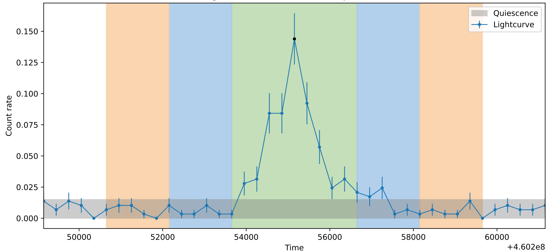
Lightcurve ObsID: 13838, Shape: None
