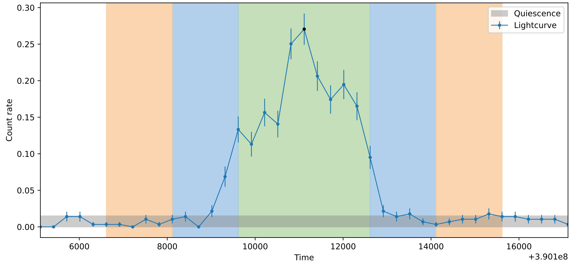
Lightcurve ObsID: 11843, Shape: None
