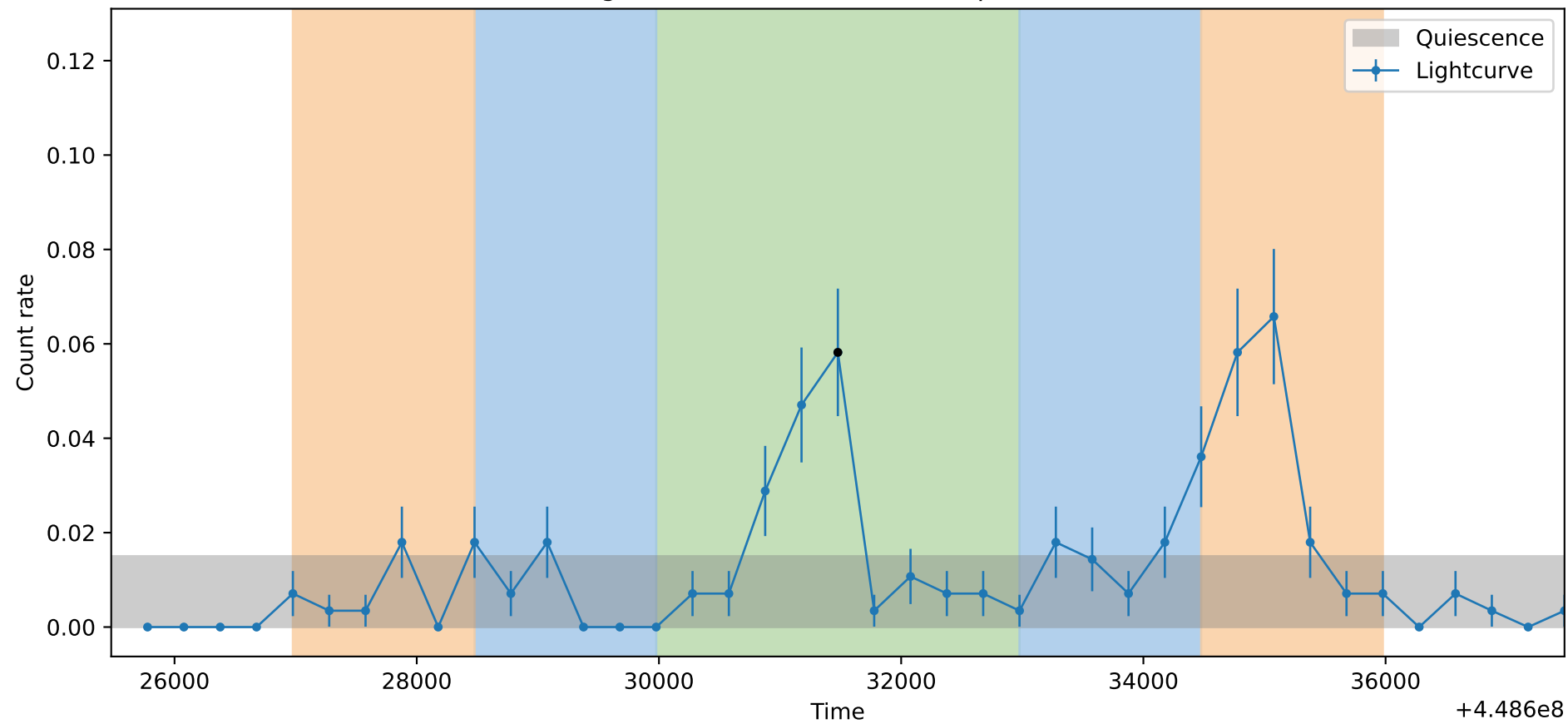
Lightcurve ObsID: 13854, Shape: None
