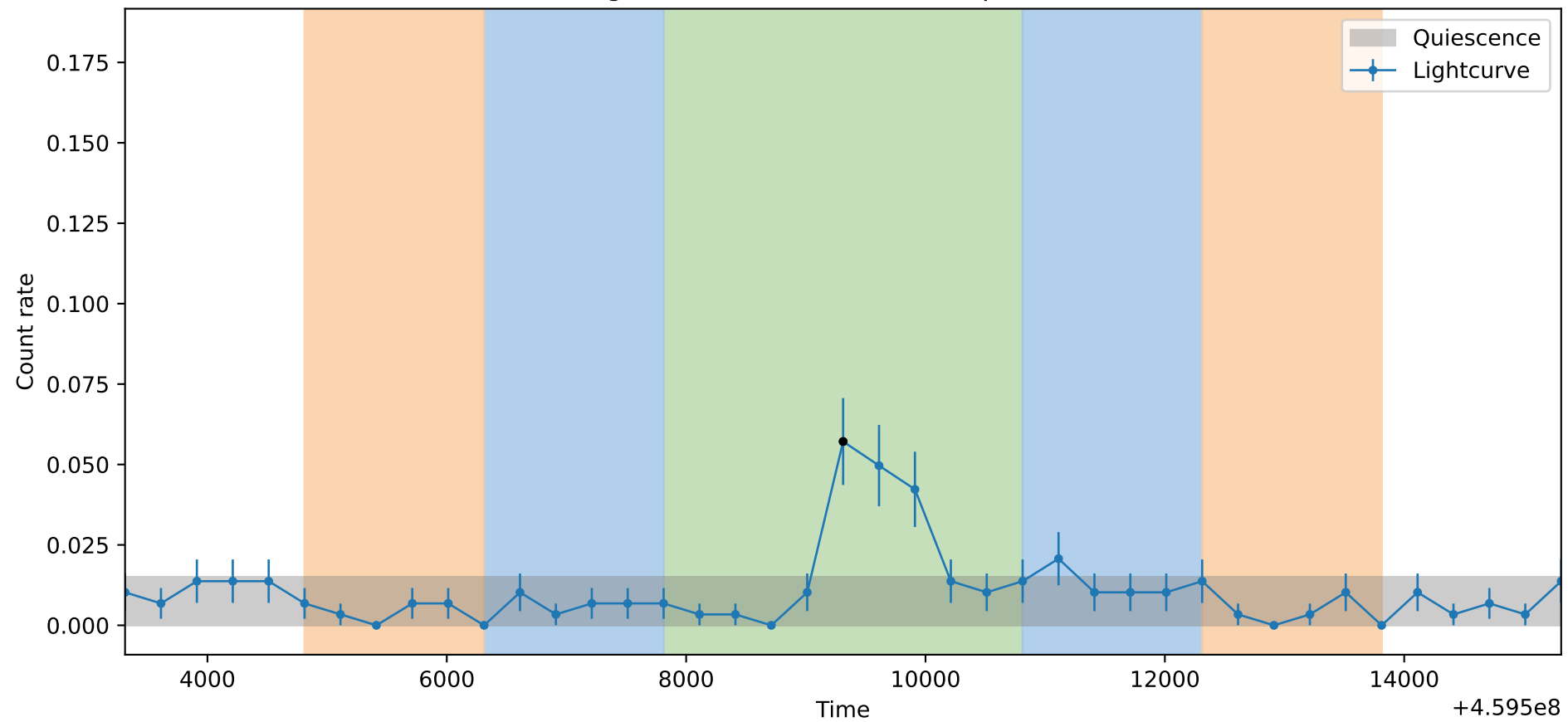
Lightcurve ObsID: 13839, Shape: None
