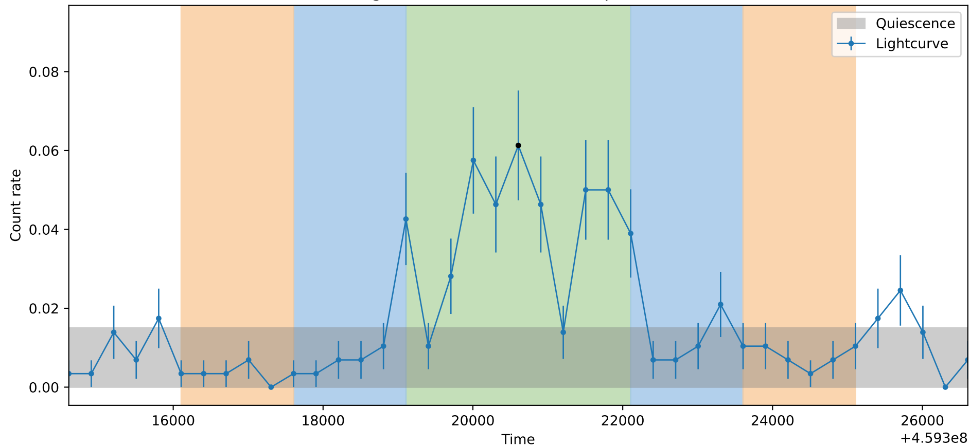
Lightcurve ObsID: 13842, Shape: None
