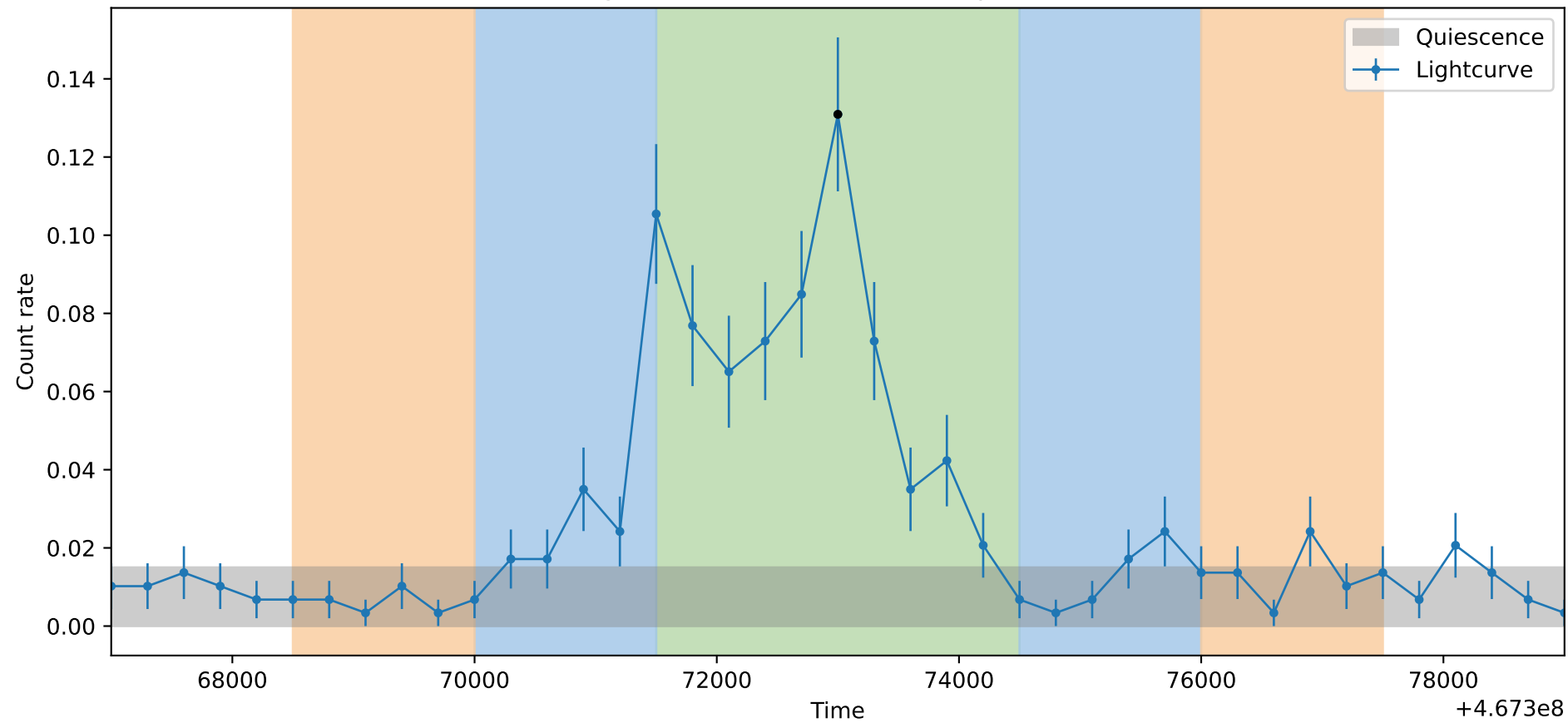
Lightcurve ObsID: 13843, Shape: None
