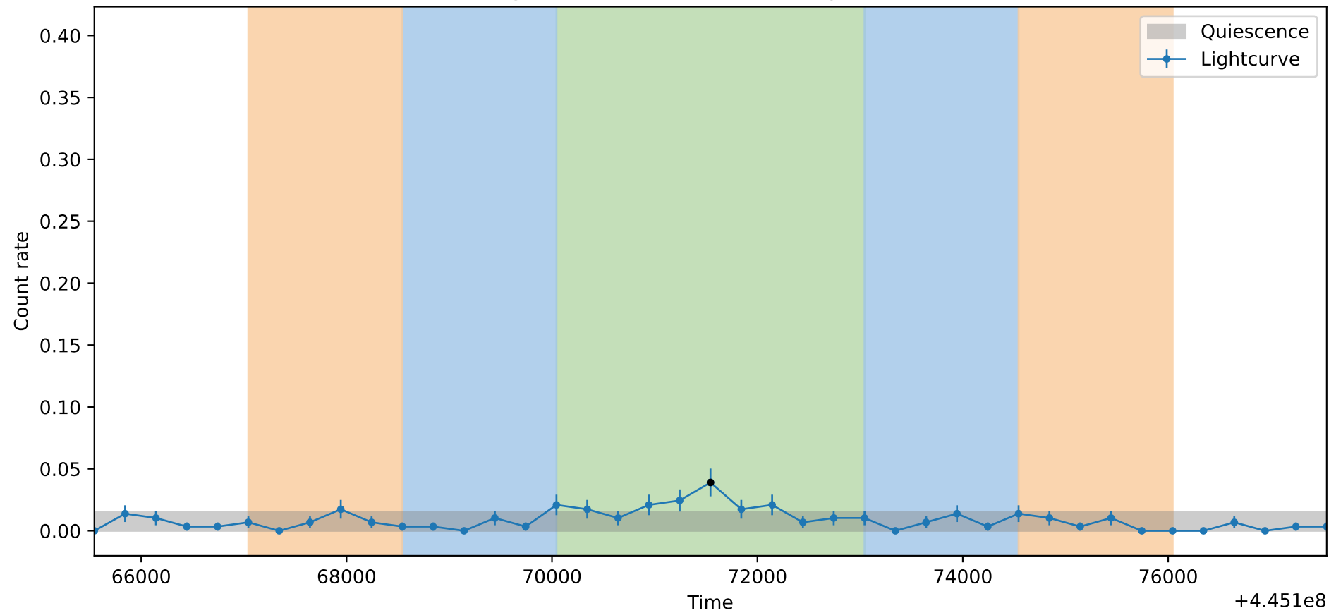
Lightcurve ObsID: 14392, Shape: None
