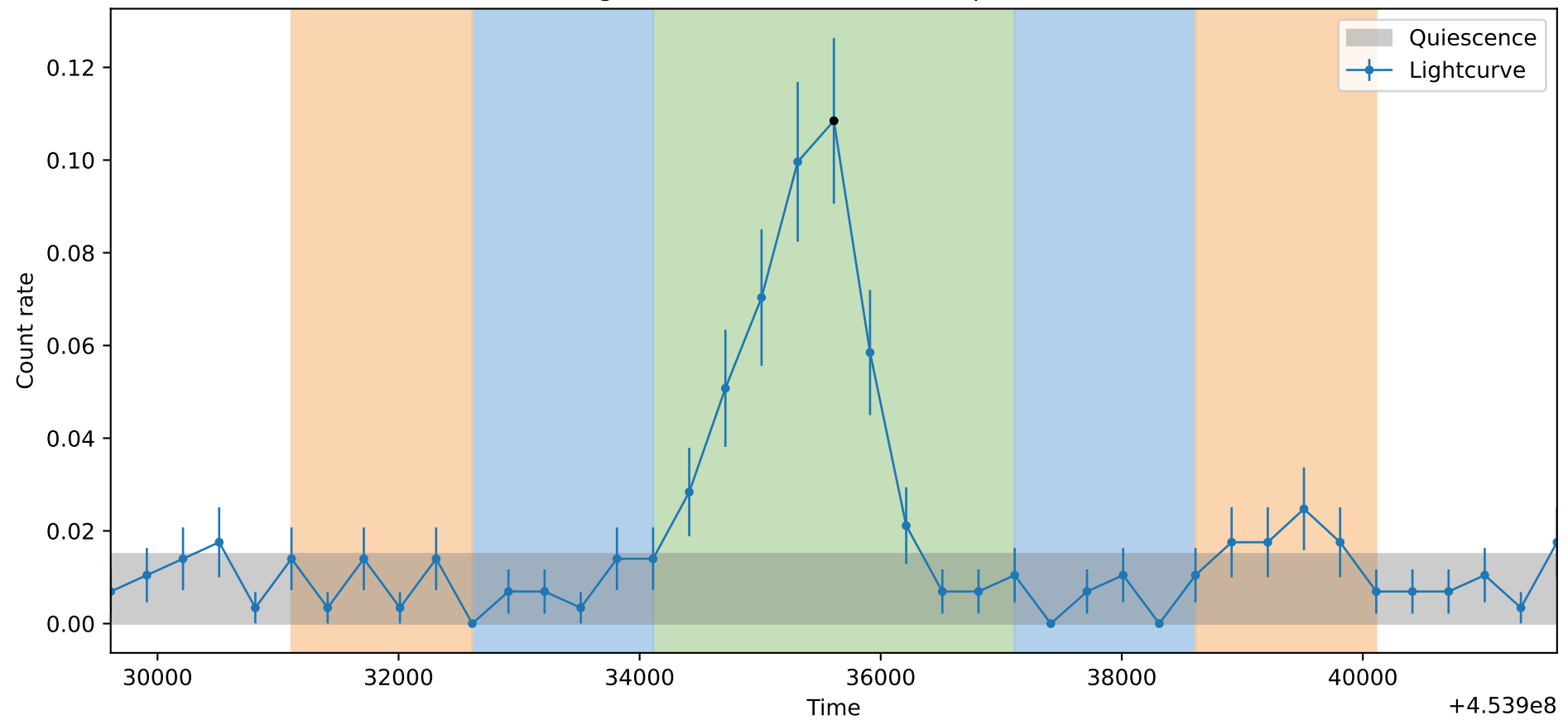
Lightcurve ObsID: 13845, Shape: None
