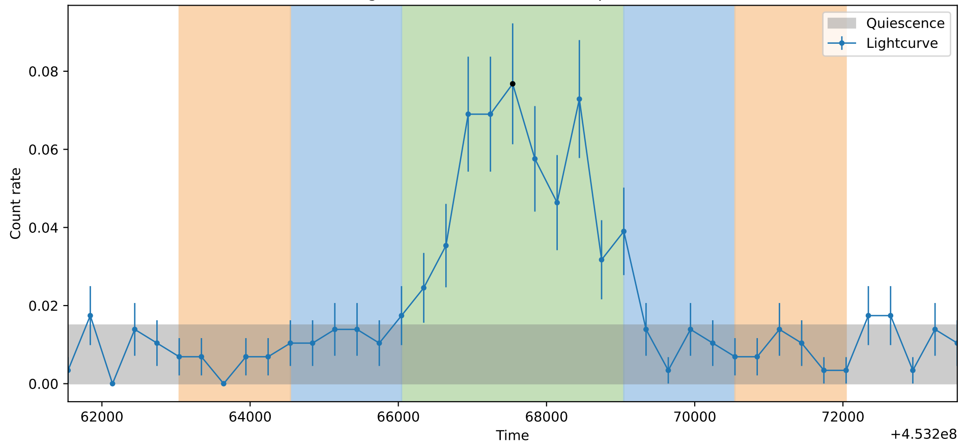
Lightcurve ObsID: 13849, Shape: None
