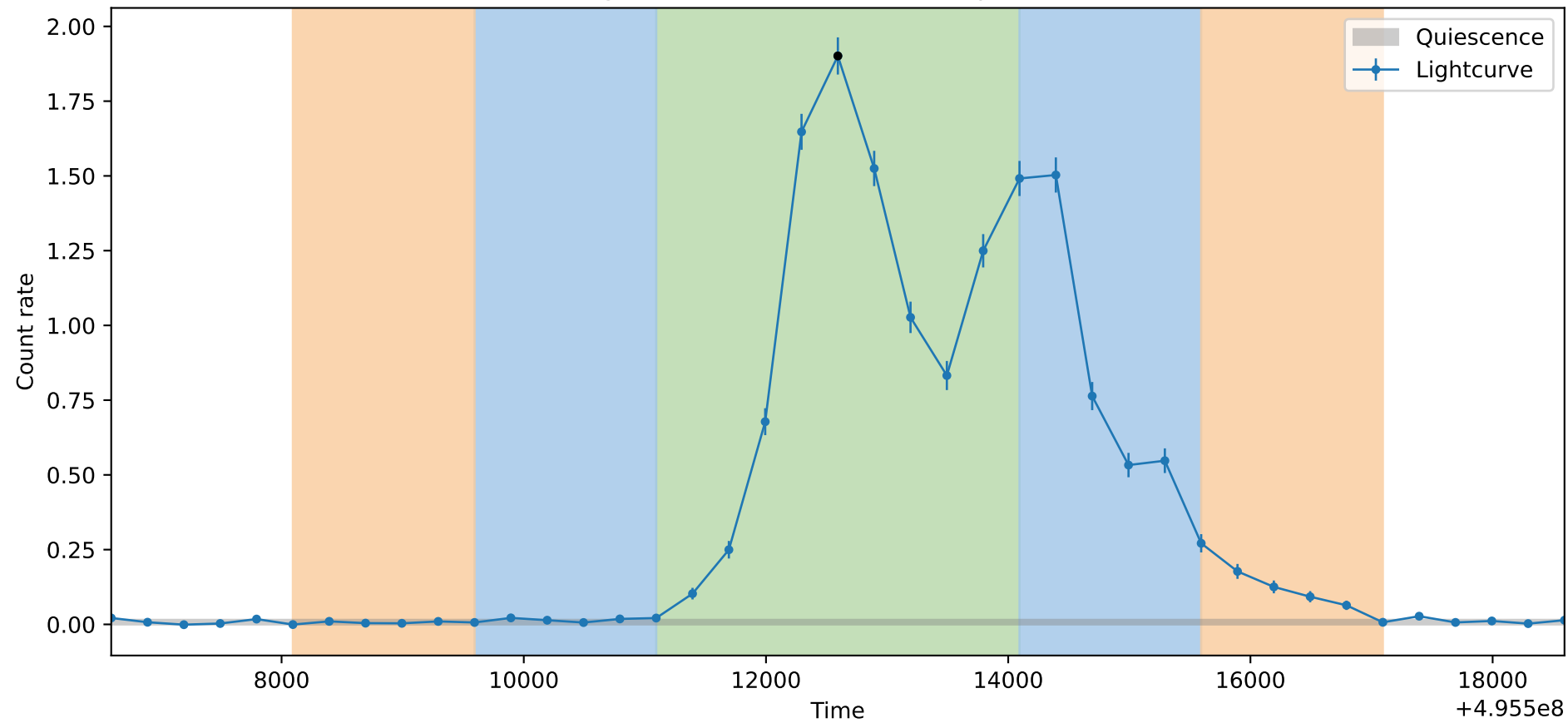
Lightcurve ObsID: 15043, Shape: None
