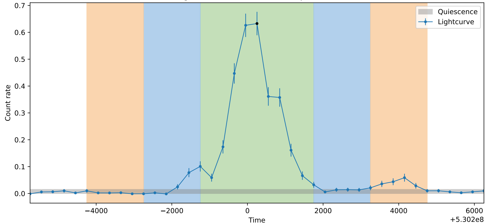
Lightcurve ObsID: 16218, Shape: None
