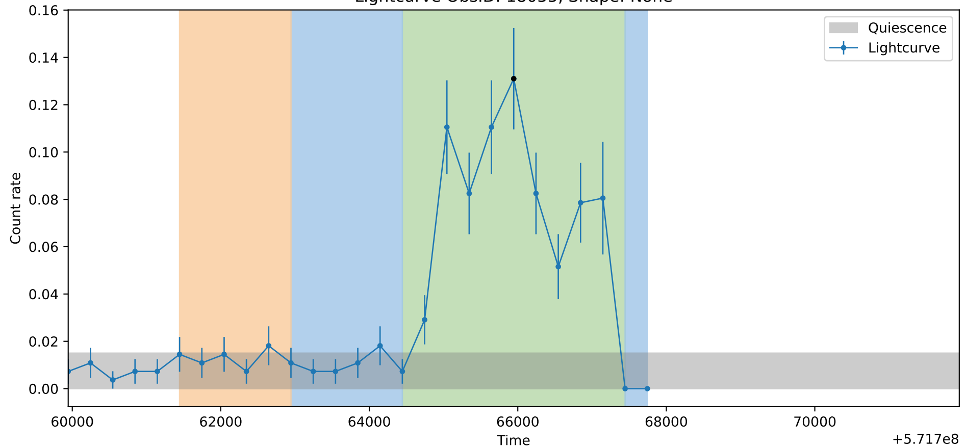
Lightcurve ObsID: 18055, Shape: None
