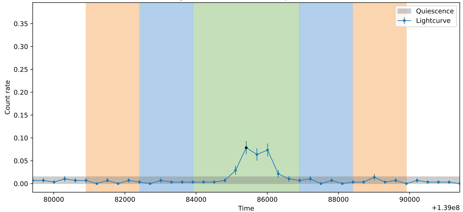
Lightcurve ObsID: 3393, Shape: None
