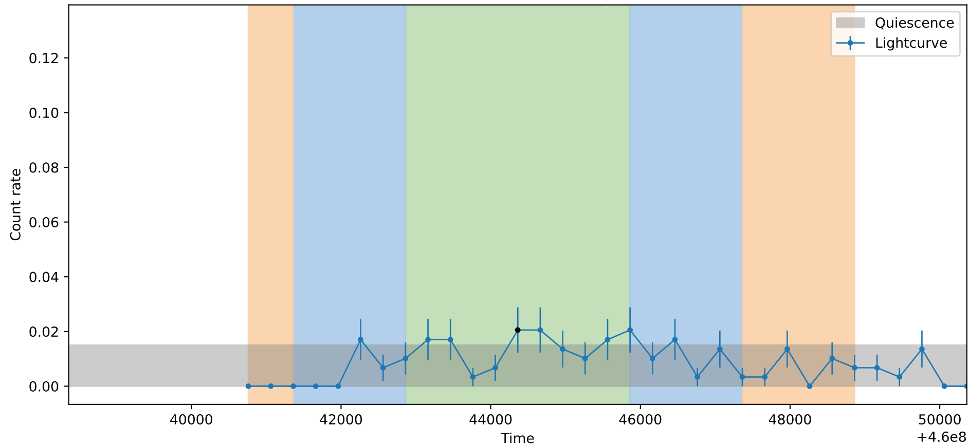
Lightcurve ObsID: 14432, Shape: None
