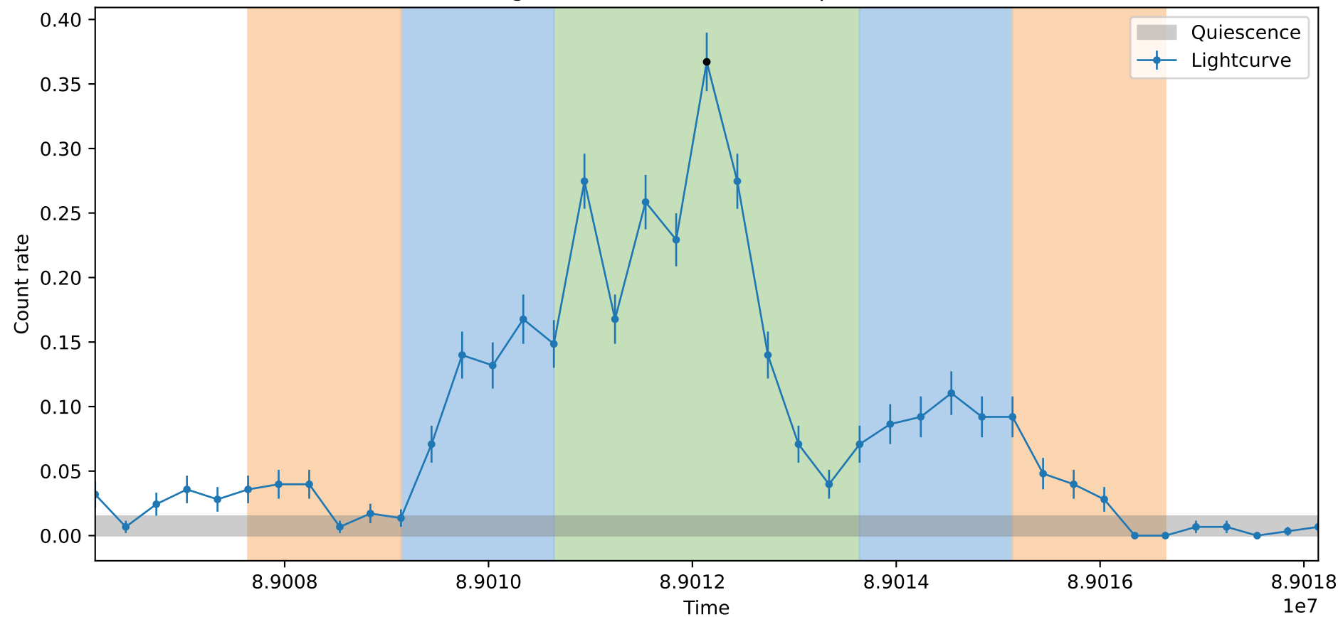
Lightcurve ObsID: 1561, Shape: None
