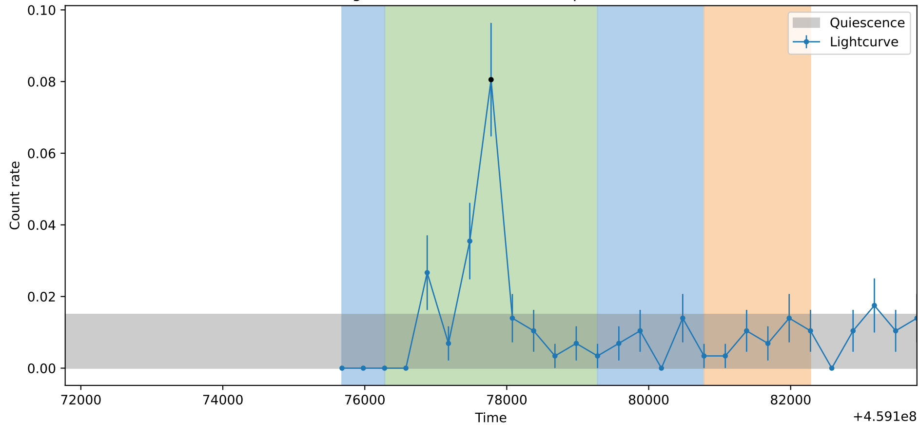
Lightcurve ObsID: 14466, Shape: None
