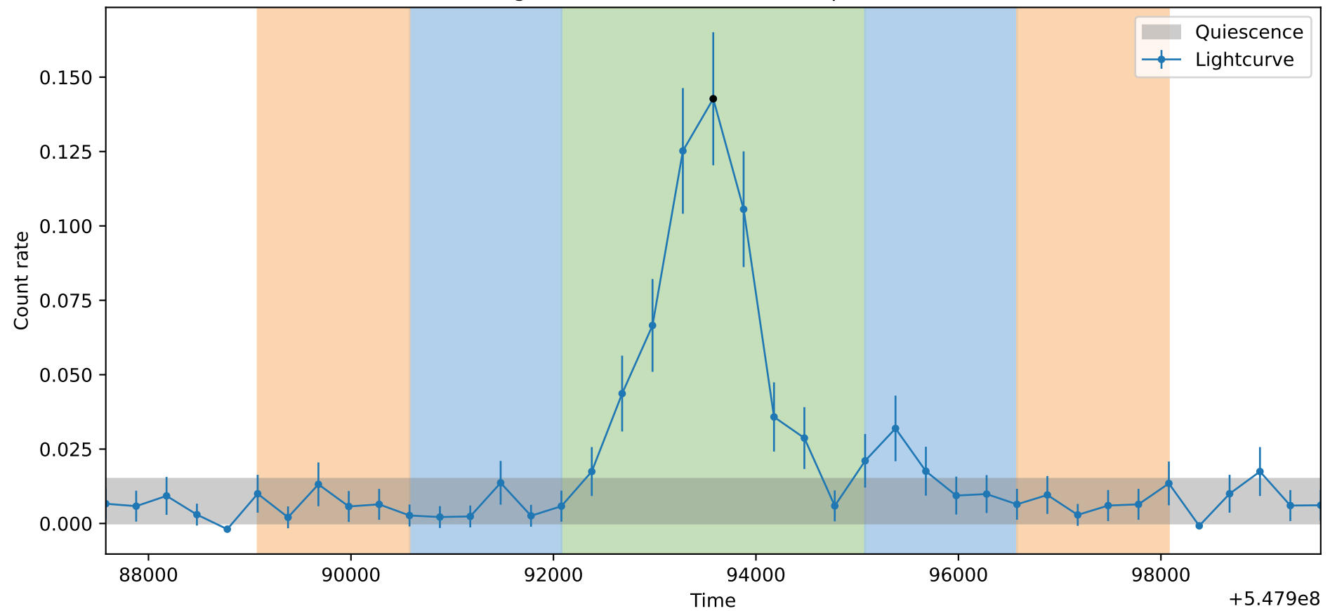
Lightcurve ObsID: 16966, Shape: None
