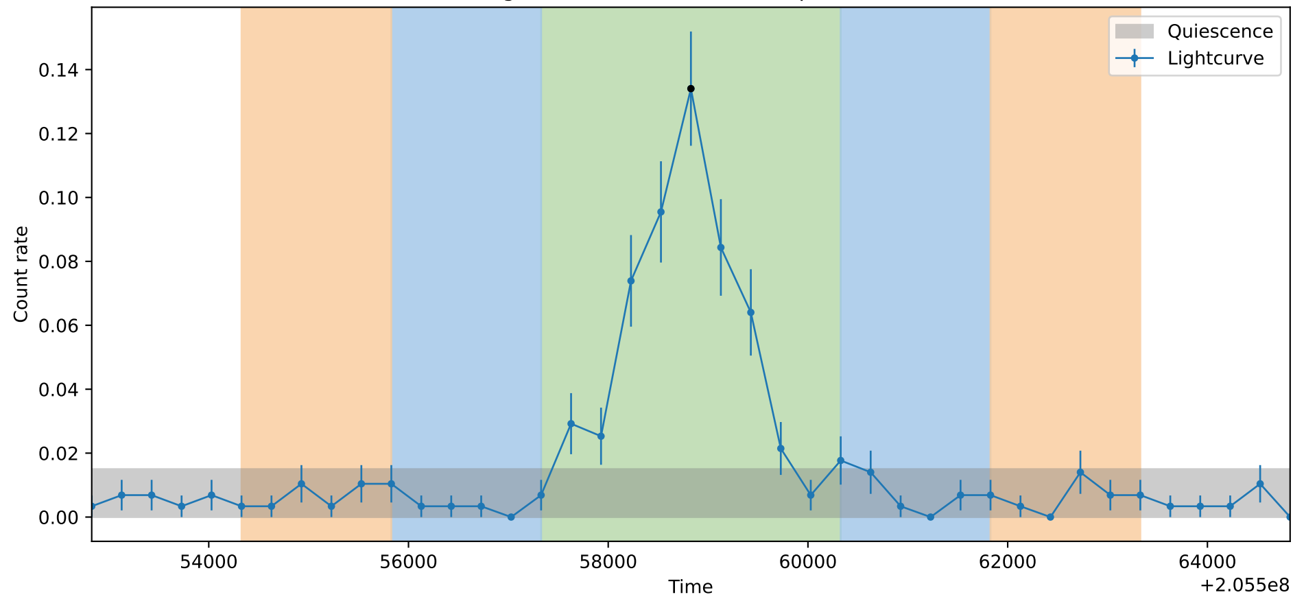
Lightcurve ObsID: 4684, Shape: None
