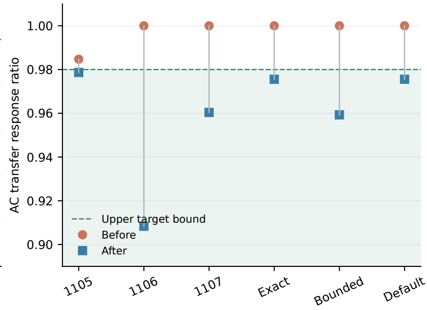
(b) Transfer target recovery
