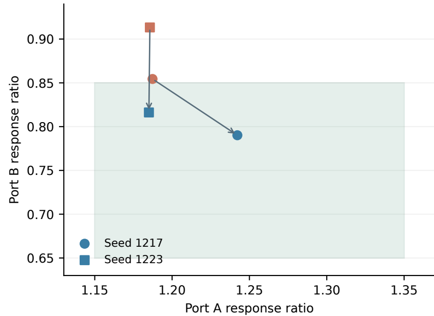
(c) Coupled target recovery
