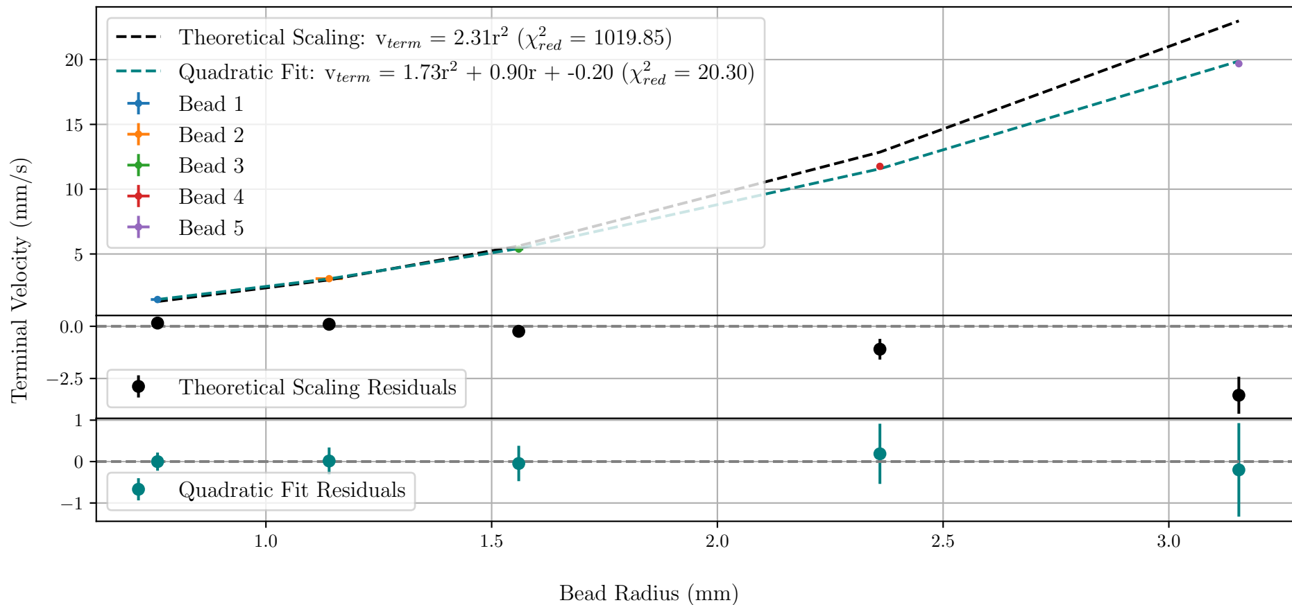
Terminal Velocity vs Bead Radius
