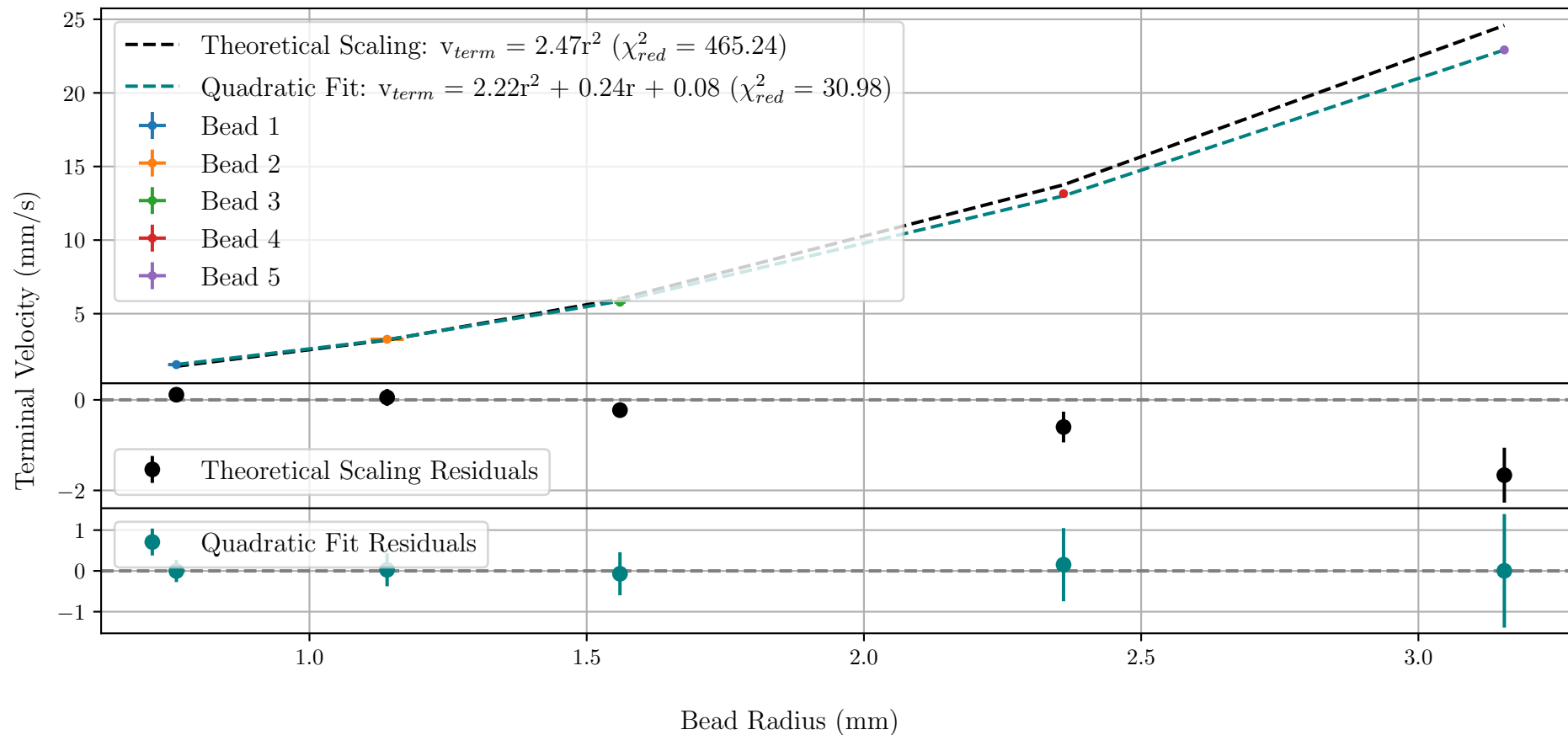
Terminal Velocity vs Bead Radius With Wall Effect Correction
