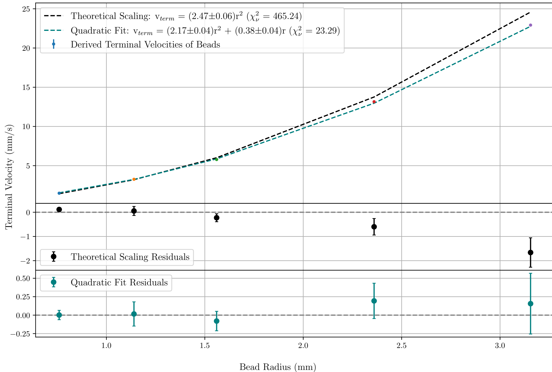
Terminal Velocity vs. Bead Radius With Wall Effect Correction Excluding Systematic Error
