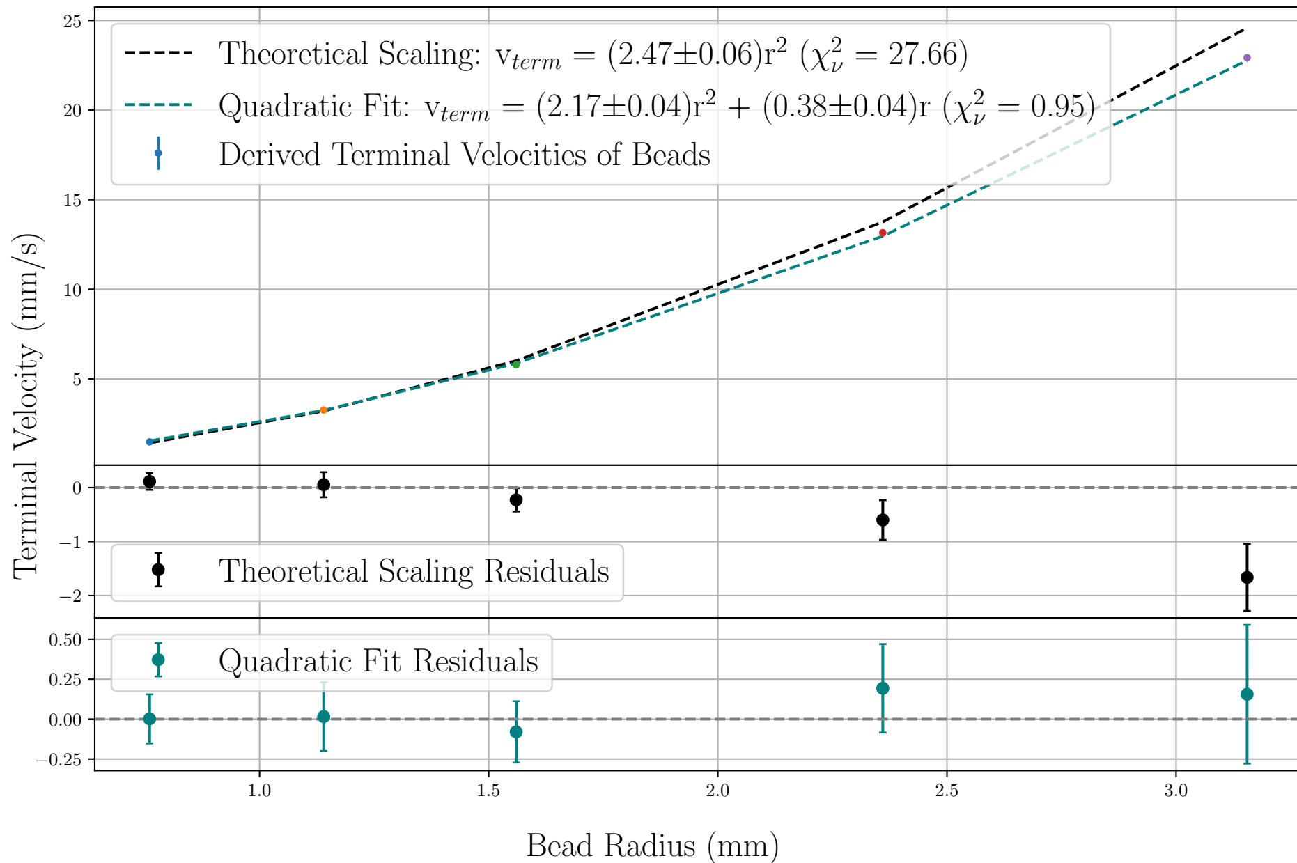
Terminal Velocity vs. Bead Radius With Wall Effect Correction
