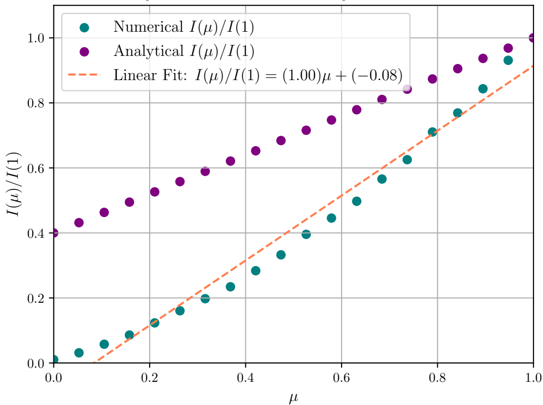
The Analytical vs. Numerical Intensity Ratio With \tau_{max} = 10
