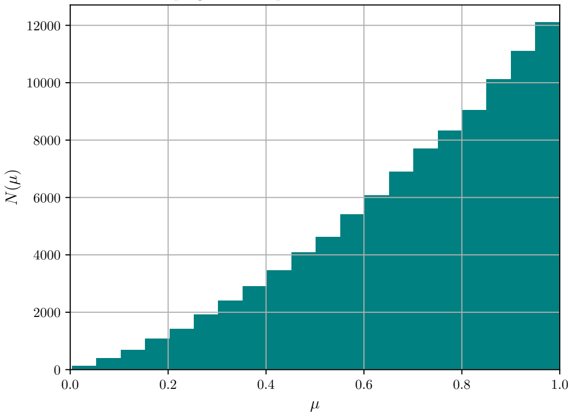
Photons Escaping With Respective Directional Cosine Distribution
