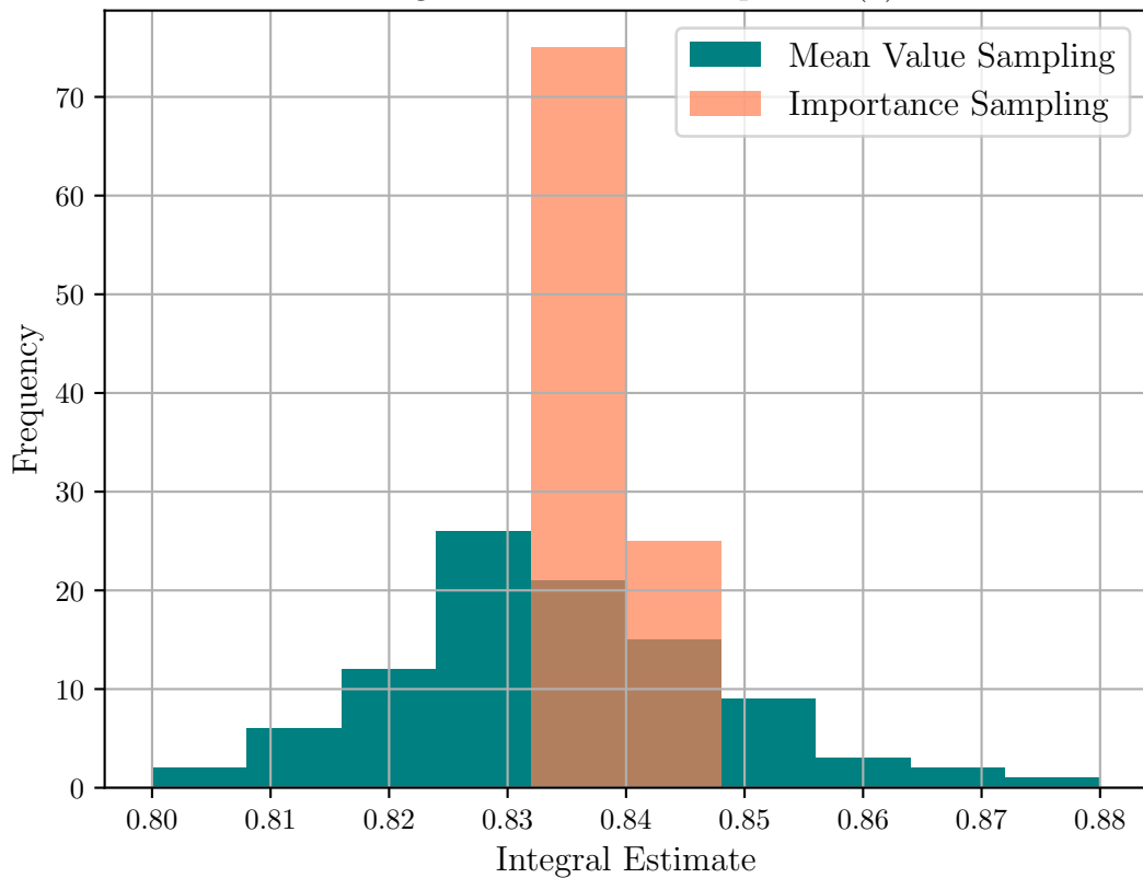
Integrand Estimates of Equation (8)
