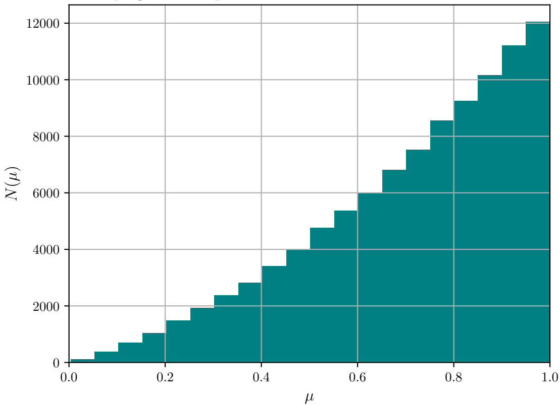
Photons Escaping With Respective Directional Cosine Distribution With \tau_{max} = 10
