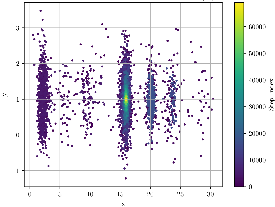
Simulated Annealing Optimization of Equation (12)
