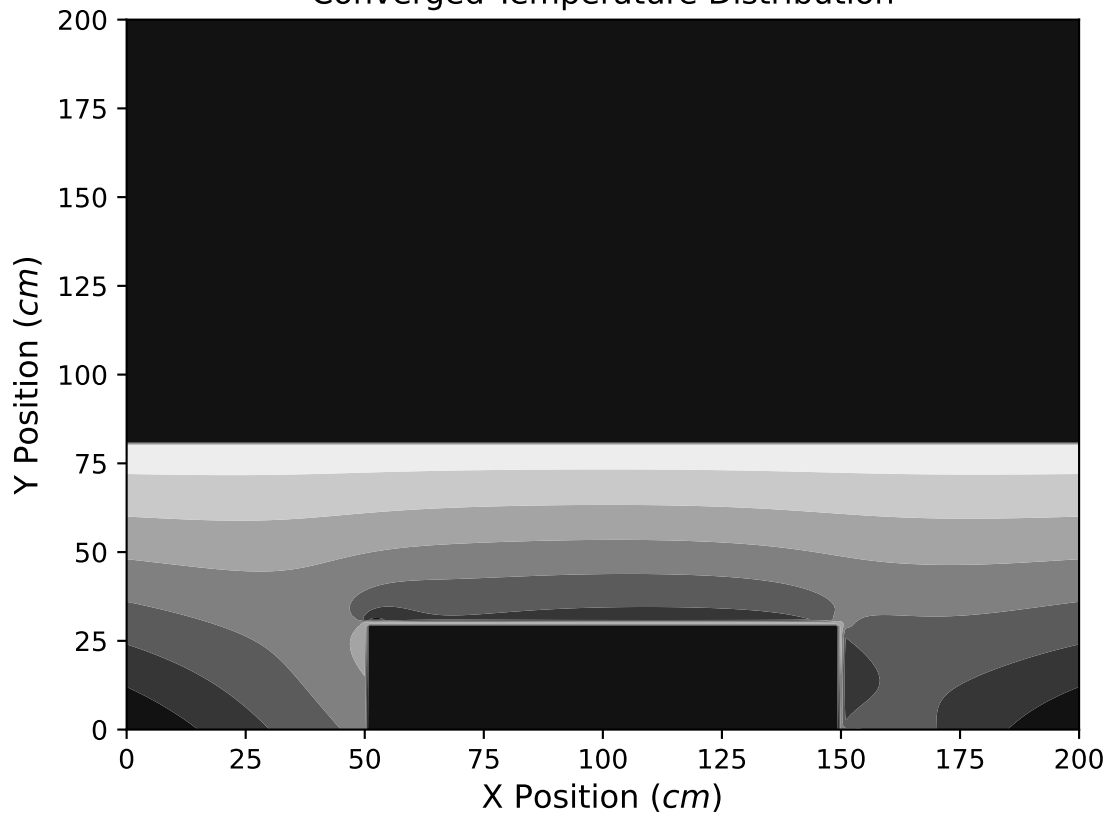
Converged Temperature Distribution
