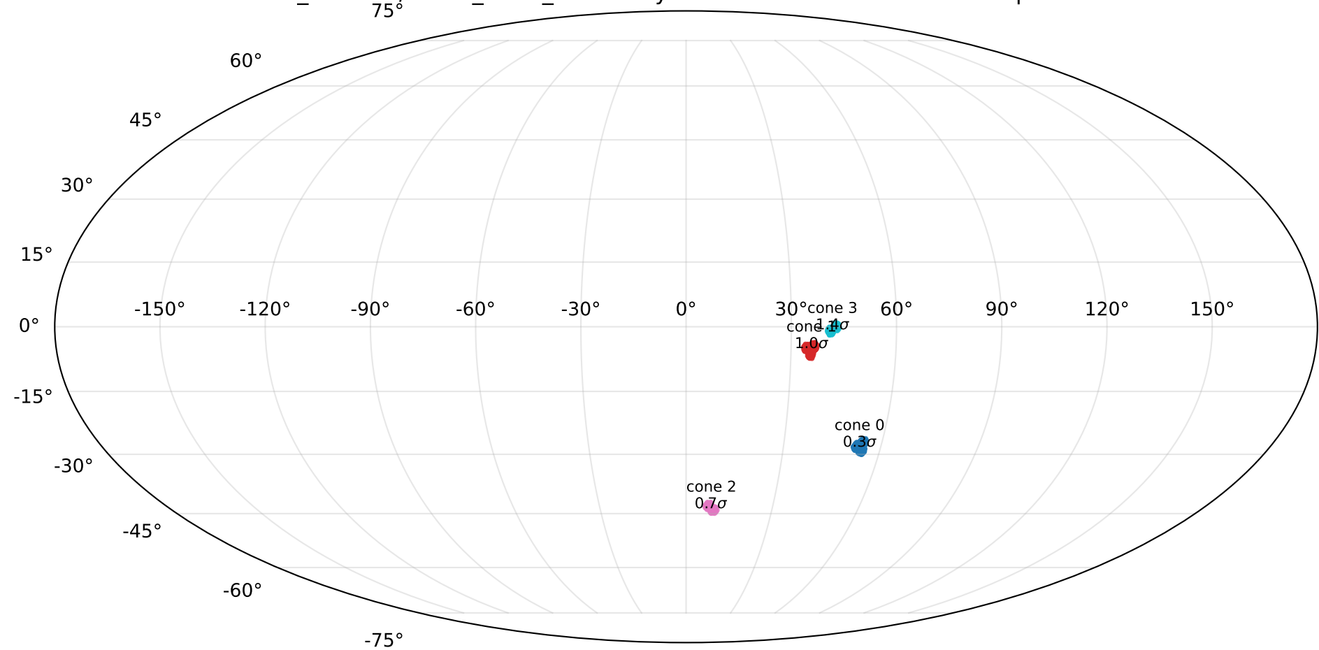
combo_ablation/cones_mass_linear: sky cones and tension vs. full-sample baseline
