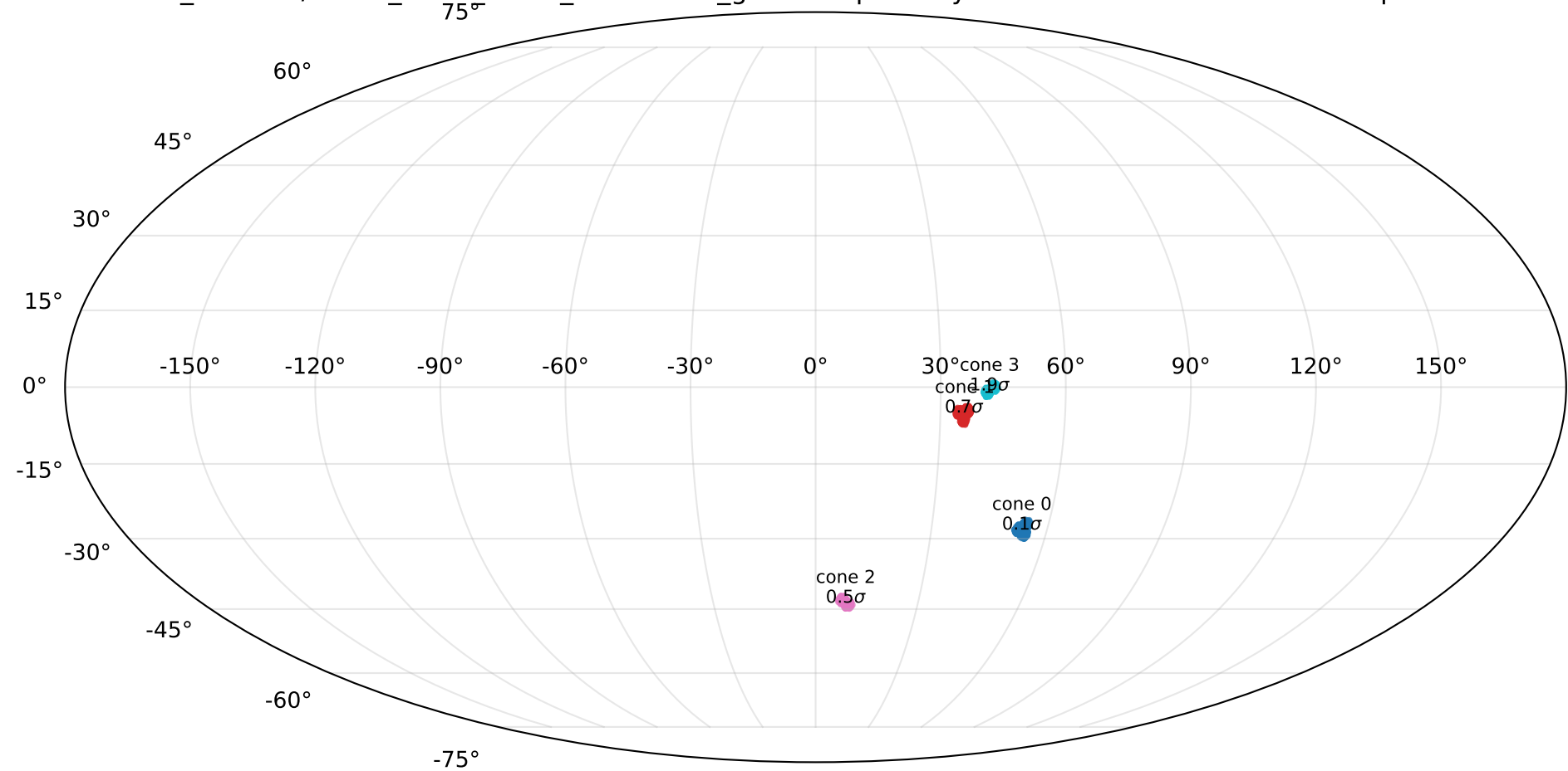
combo_ablation/cones_mass_linear_interaction_gammaalpha: sky cones and tension vs. full-sample baseline
