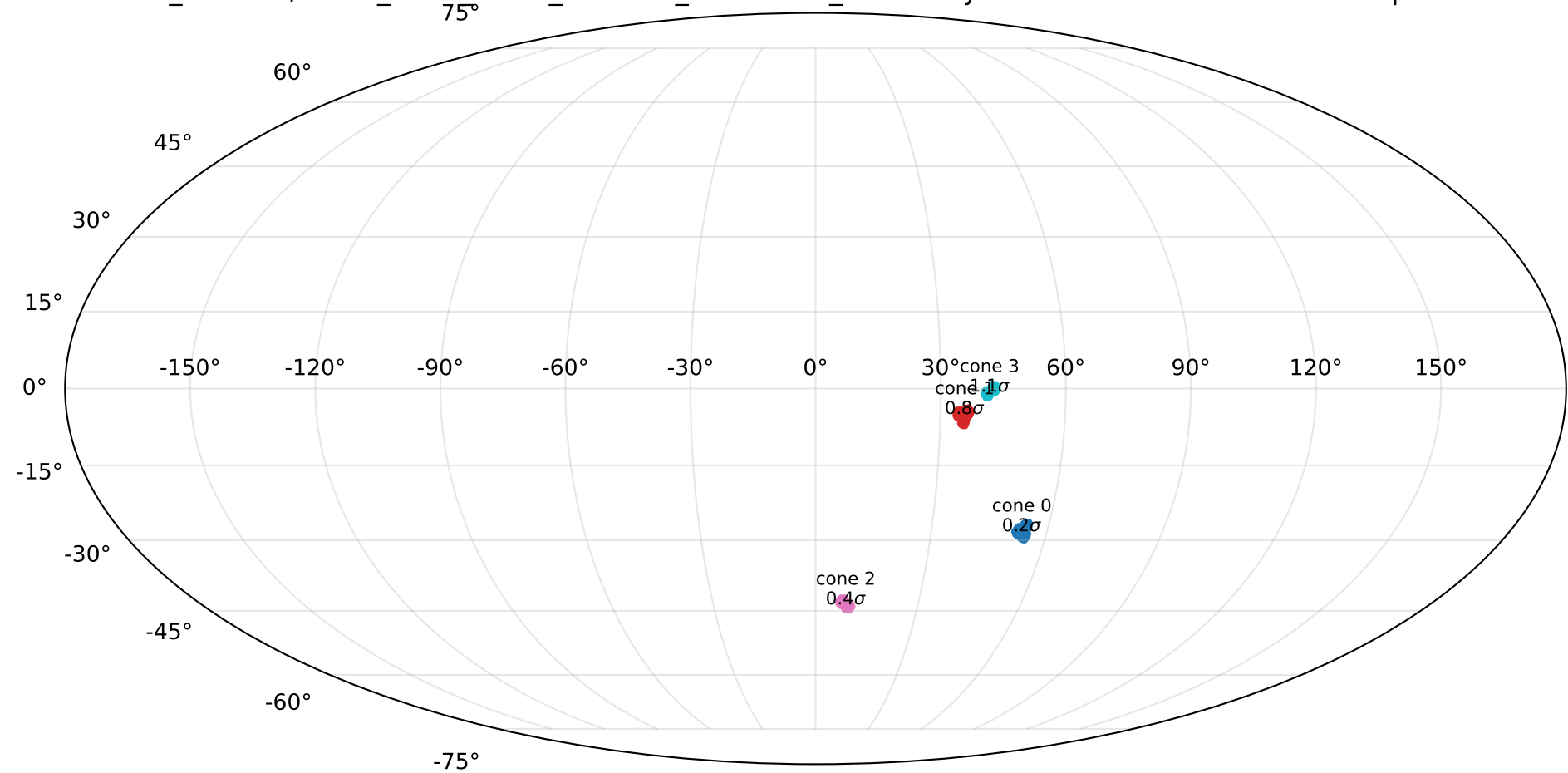
combo_ablation/cones_mass_linear_sncolour_softbroken_sntau: sky cones and tension vs. full-sample baseline
