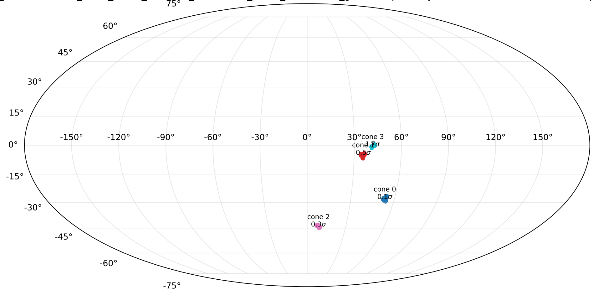
combo_ablation/cones_mass_linear_sncolour_softbroken_sntau_interaction_gammaalpha: sky cones and tension vs. full-sample baseline
