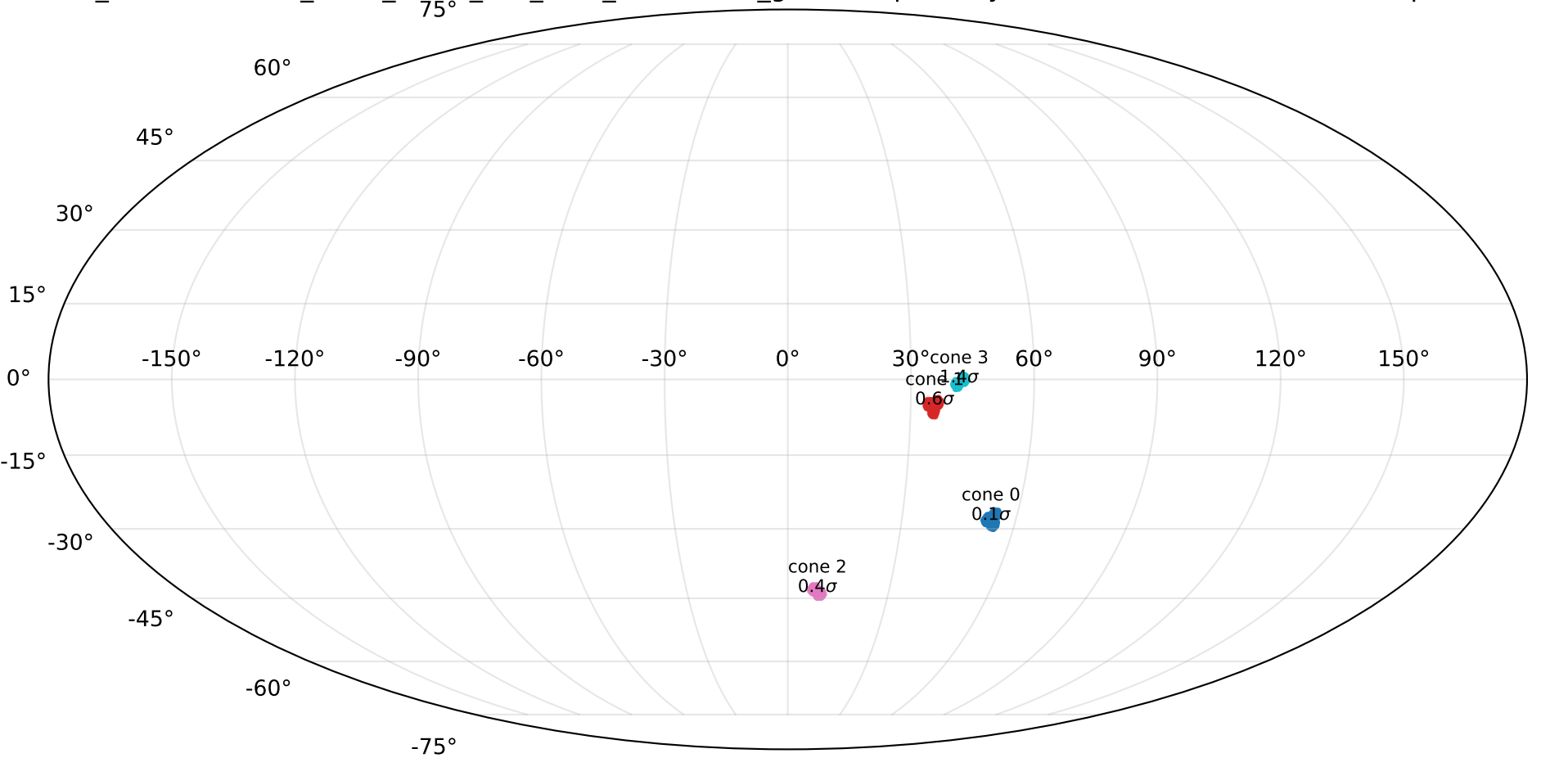
combo_ablation/cones_mass_linear_ssfr_tanh_interaction_gammaalpha: sky cones and tension vs. full-sample baseline
