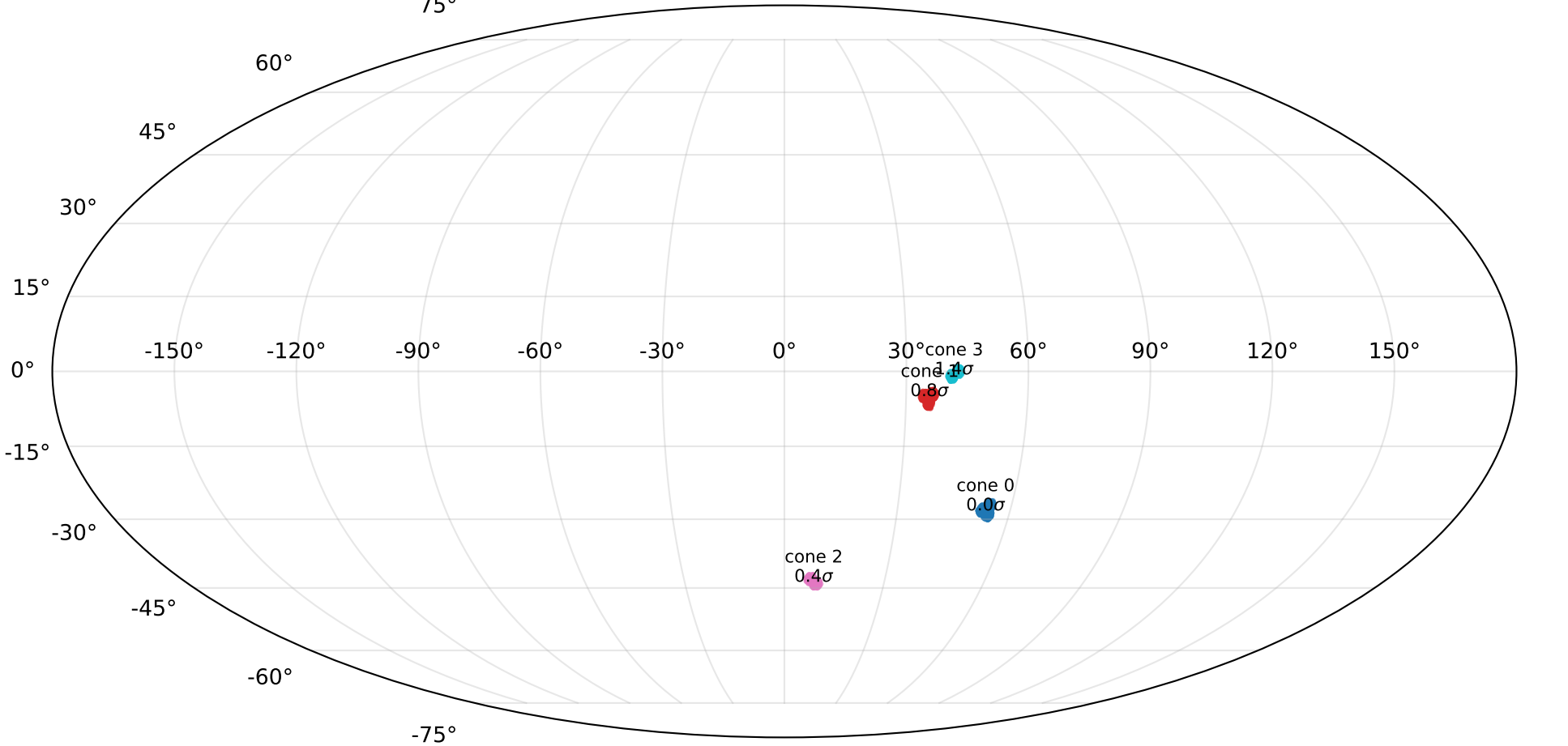
combo_ablation/cones_mass_linear_ssfr_tanh_sncolour_softbroken_sntau: sky cones and tension vs. full-sample baseline
