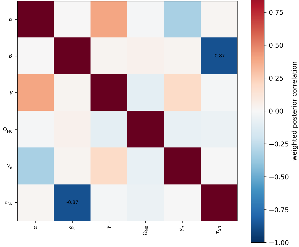
combo_ablation/deg_mass_linear_sncolour_softbroken_sntau_interaction_gammaalpha: posterior correlation (lagged threshold |r| \geq 0.85 )
