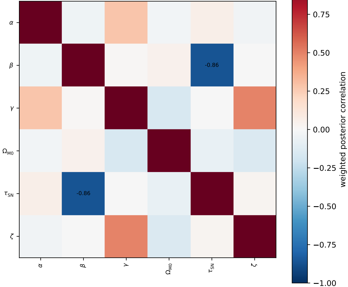
combo_ablation/deg_mass_linear_ssfr_tanh_sncolour_softbroken_sntau: posterior correlation (flagged threshold |r| \geq 0.85 )
