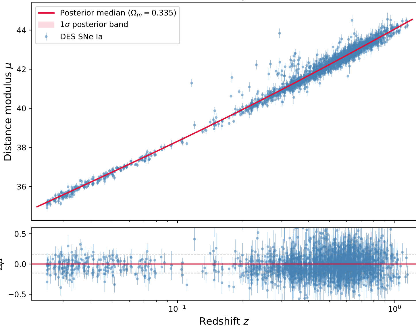
Hubble Diagram
