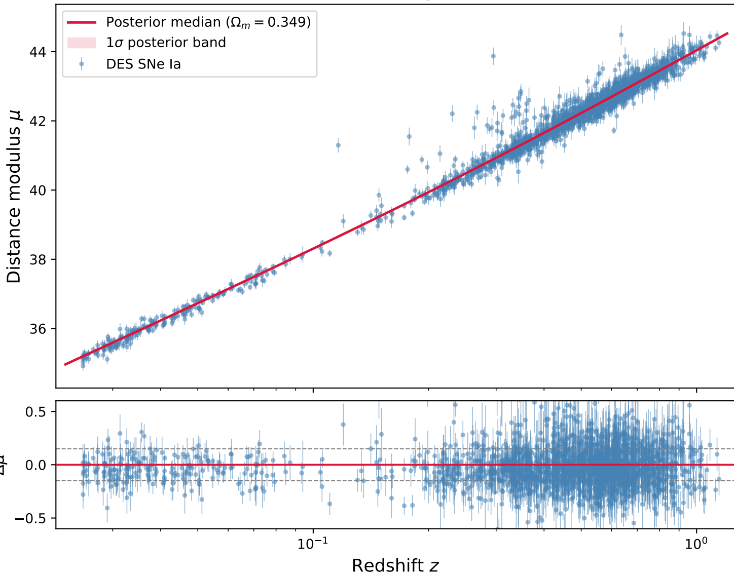
Hubble Diagram
