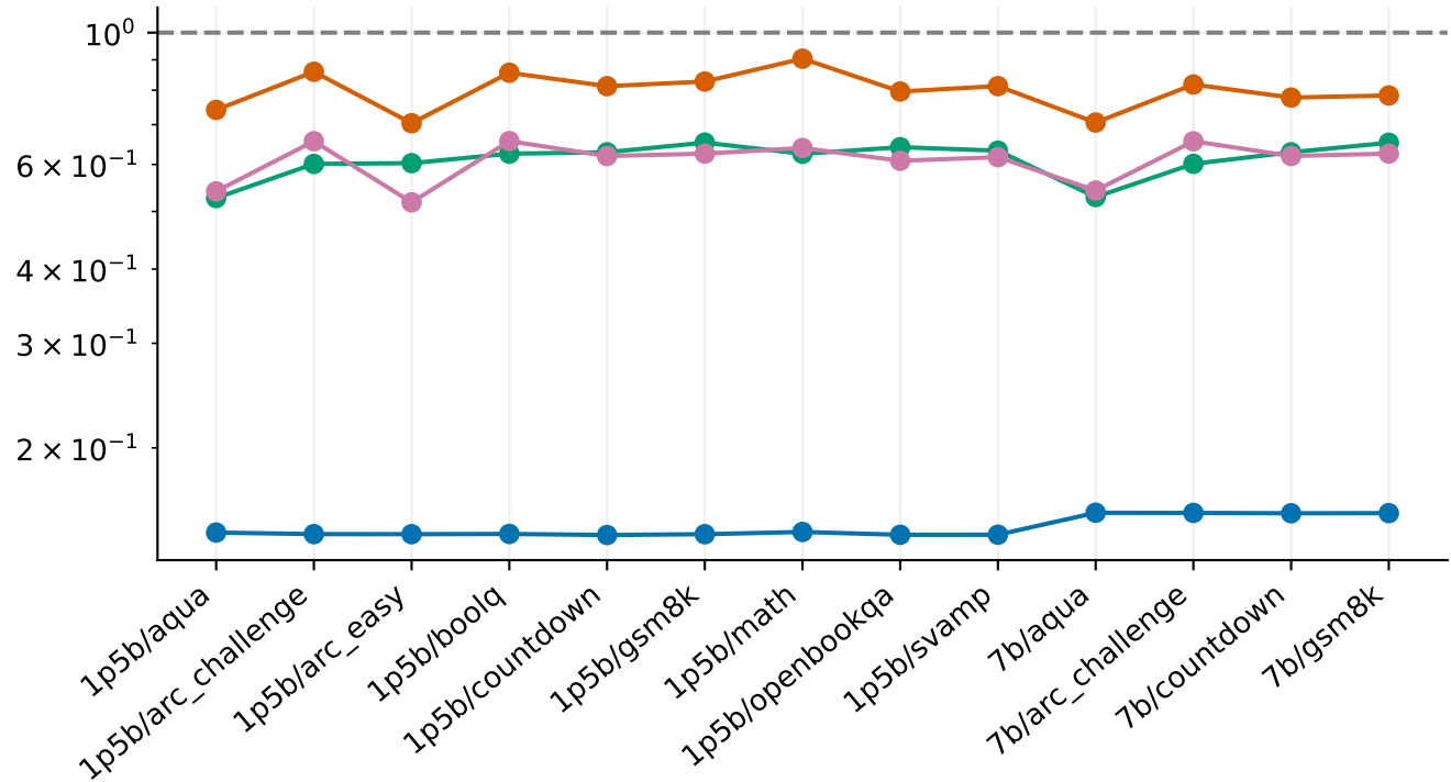
Counted arithmetic FLOPs / Oracle32
