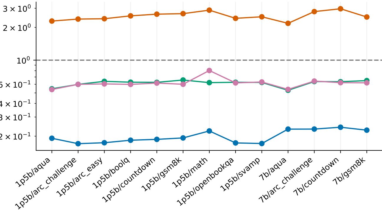
Measured online time / Oracle32
