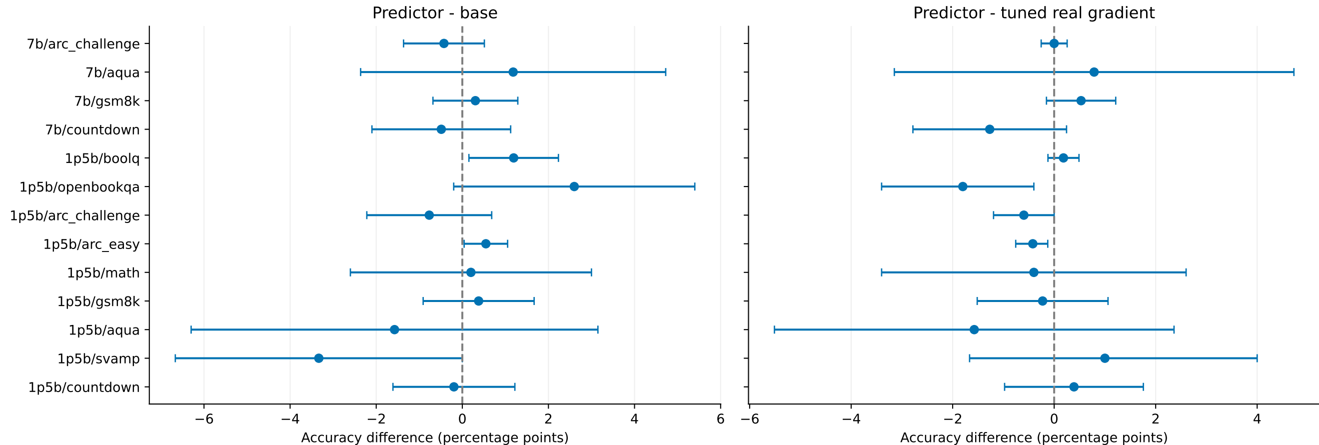
Pointwise paired-question 95% intervals (unadjusted); conditional on fitted runs
