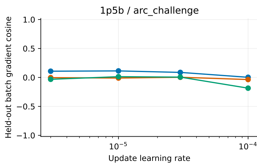
Post-update32 gradient audit; separate trajectories, no audit feedback
