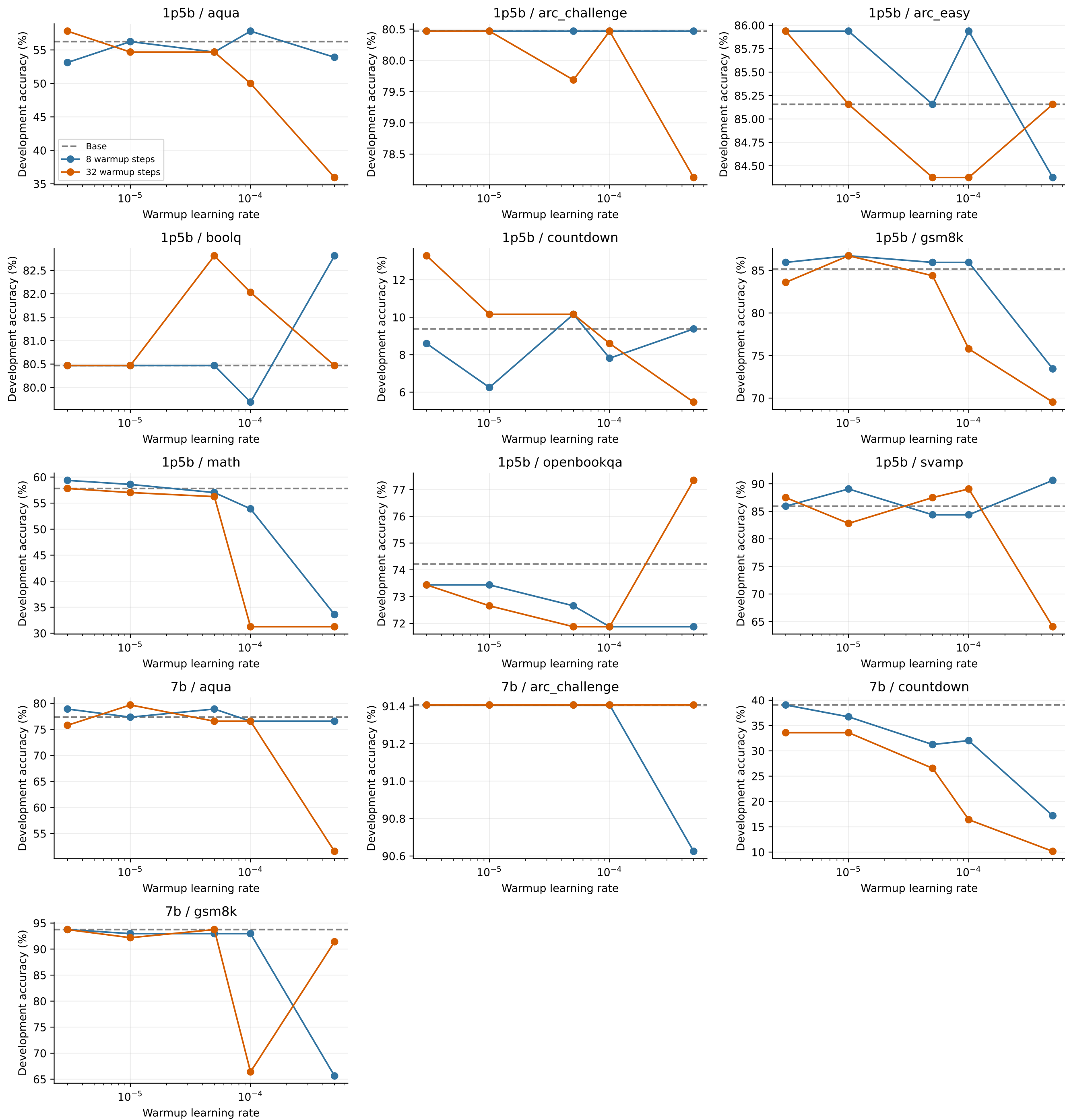
Warmup sensitivity: development set, not held-out final evidence
