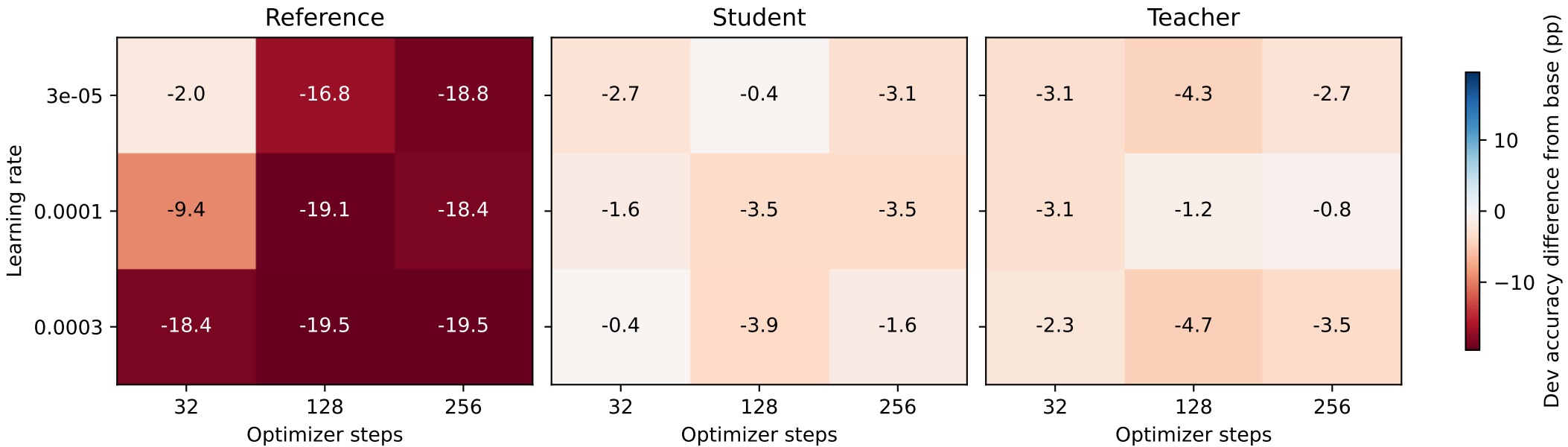
Development sensitivity: 256 questions, seed 101; base 86.72%
