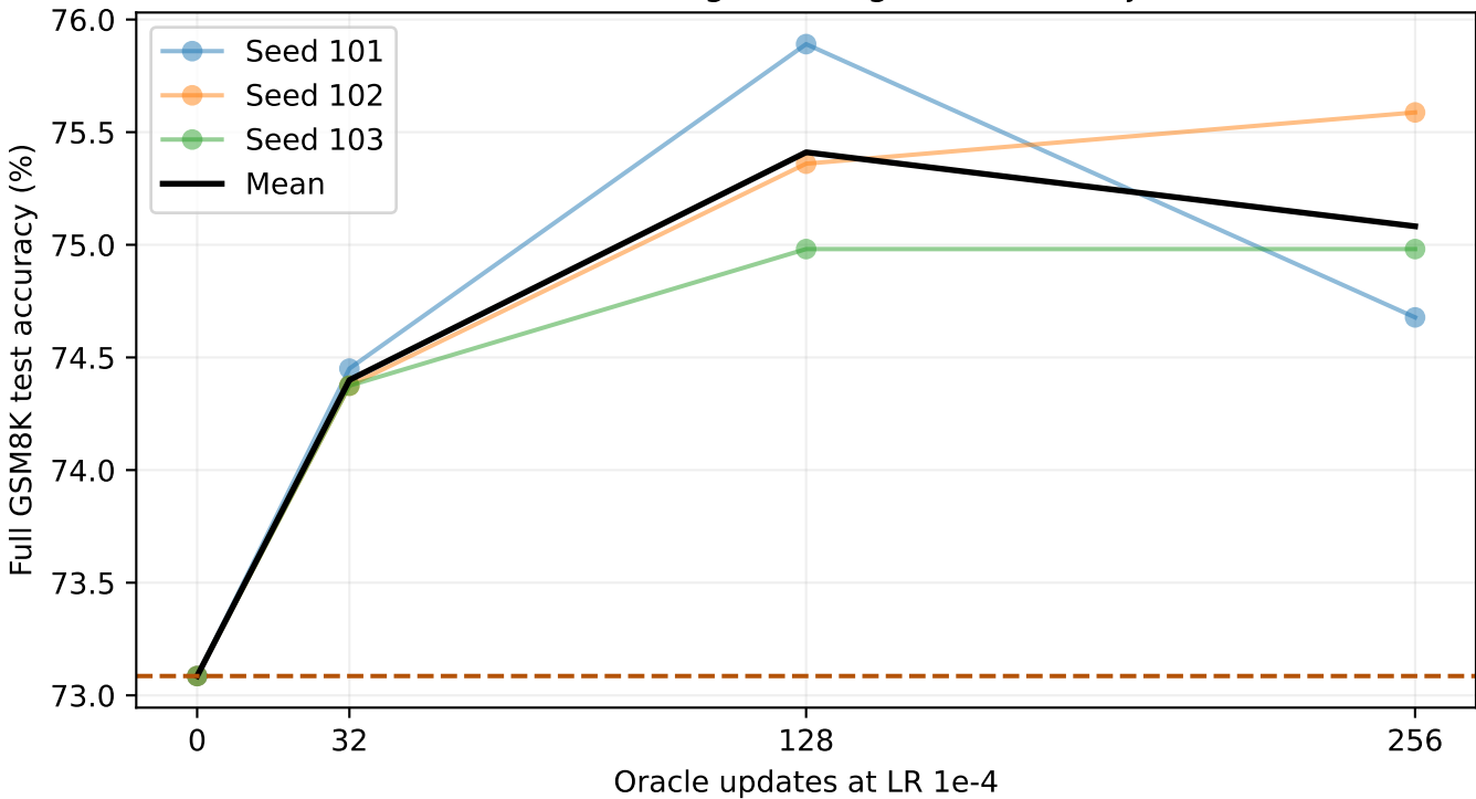
Post-hoc: teacher targets along the same trajectories
