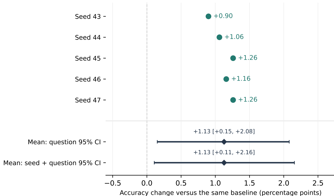
MATH test: 5,000 questions (historically reused)
