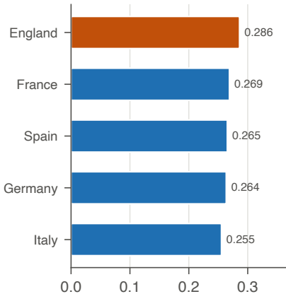
Silhouette
