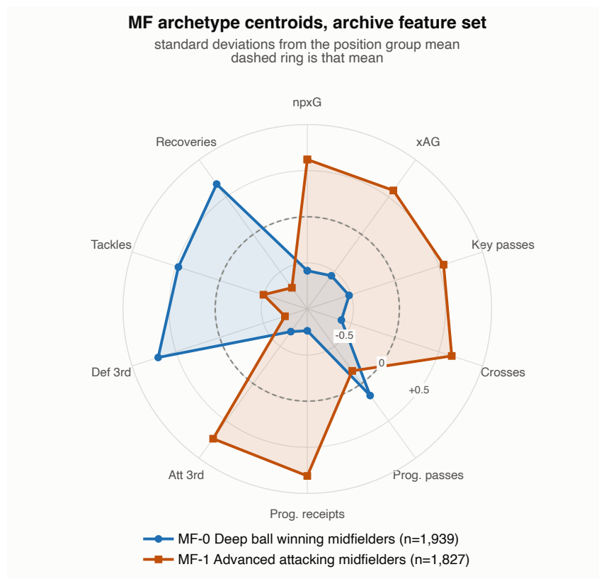
Figure 24: Midfielder archetypes, archive sample.
