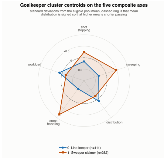
Figure 16: Goalkeeper structure on the primary sample. The clusters separate on off-line activity; distribution and shot stopping vary continuously across both.
