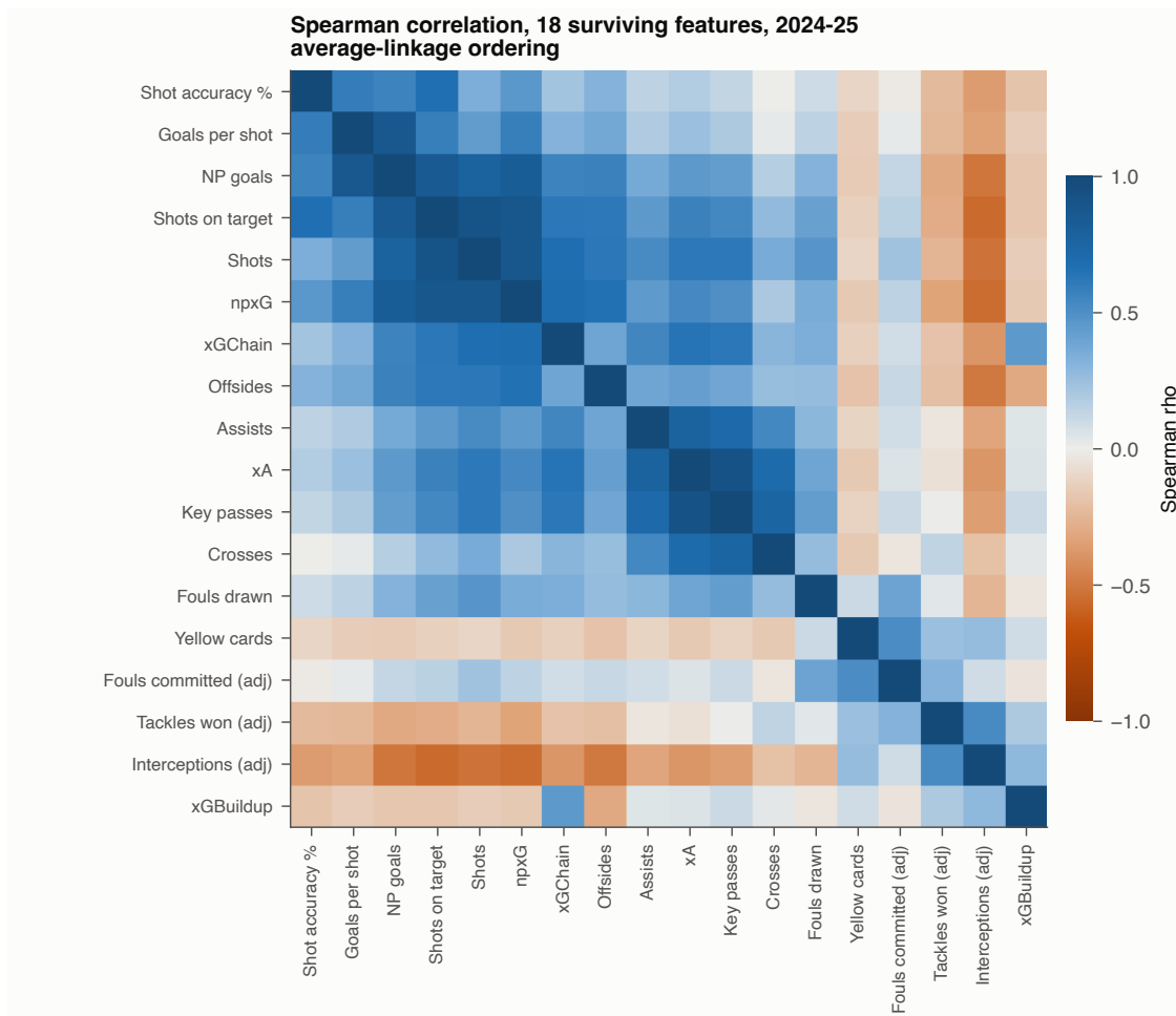
Figure 19: Hierarchically clustered Spearman correlation matrix over the outfield feature set in the earlier of the two reduced-sample seasons.
