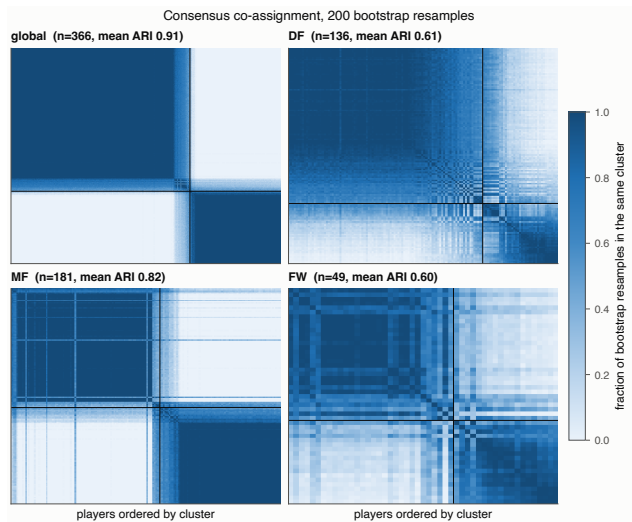
(a) Bootstrap co-assignment.
