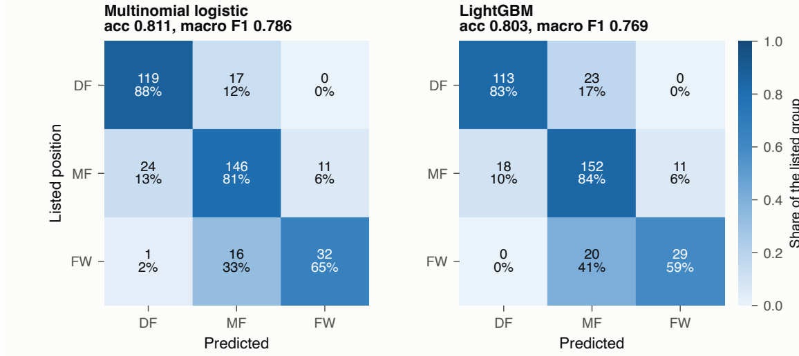
(a) Confusion between listed positions.
