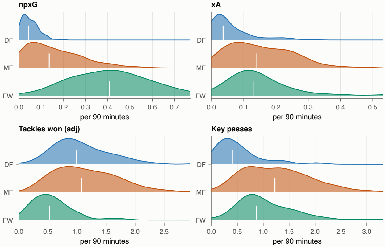
Figure 32: Distributions of four representative per-90 statistics across position groups in the earlier of the two reduced-sample seasons. The separation between groups is clear for shot volume and for defensive actions, and much weaker for creation.
