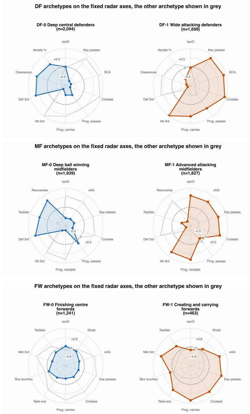
Figure 5: Archetype radars on fixed axes within each position group.
