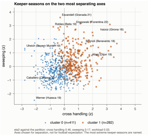
(b) Distribution of the archive goalkeeper composites.
