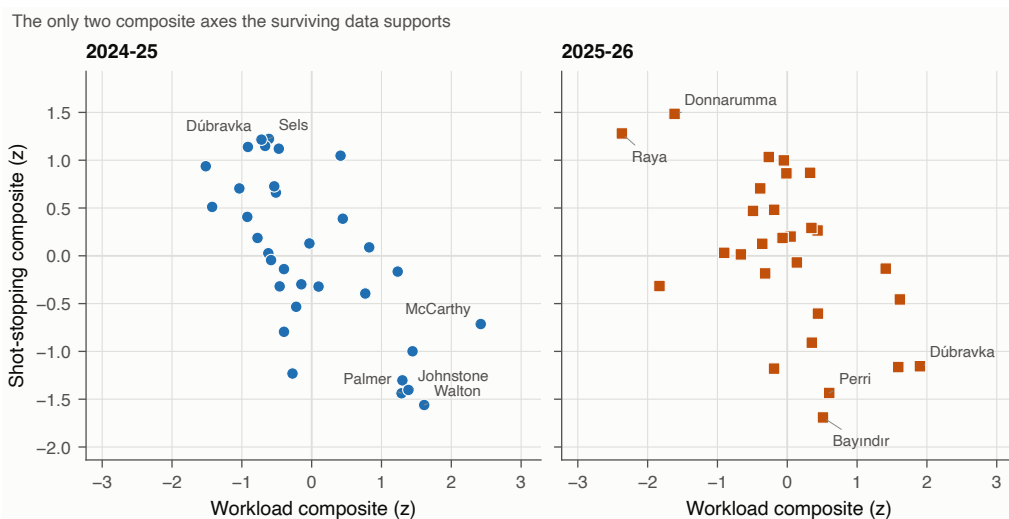
(b) The two surviving composite axes.
