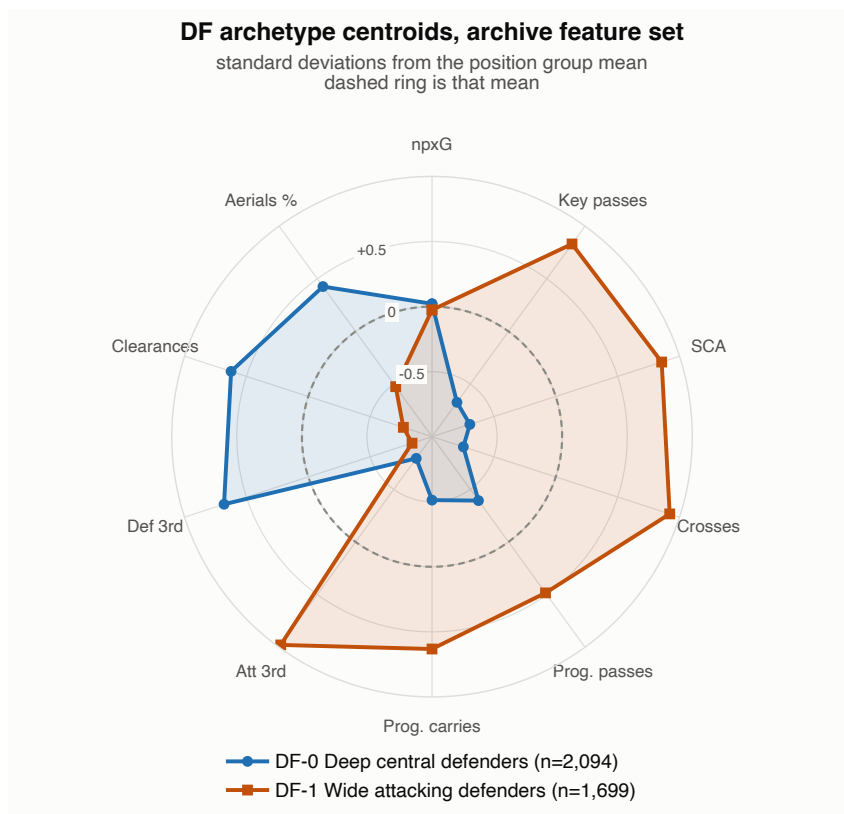
Figure 23: Defender archetypes, archive sample.
