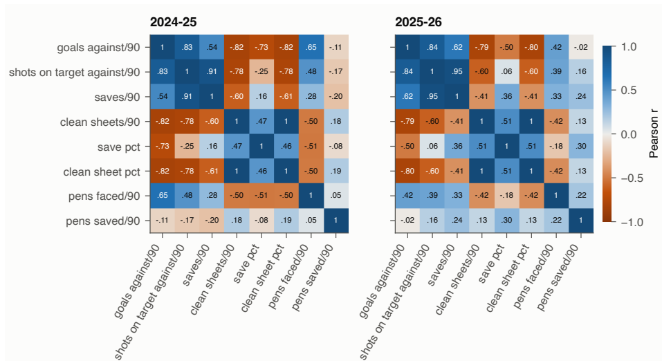
(a) Surviving goalkeeper features.
