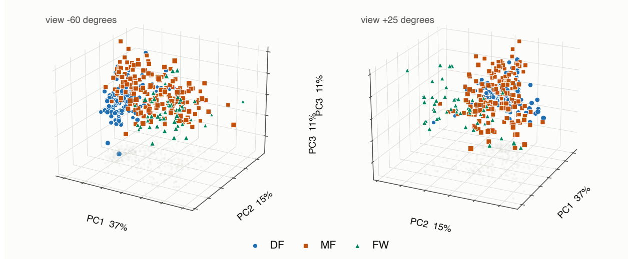
Figure 34: Outfield players in the first three principal components, from two viewpoints. Grey points on the floor are the vertical projection of each player, supplying a depth cue that a static rendering otherwise lacks.
