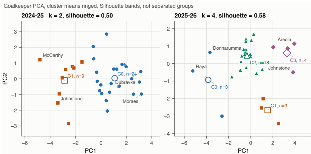
(a) Goalkeeper clusters in principal component space.
