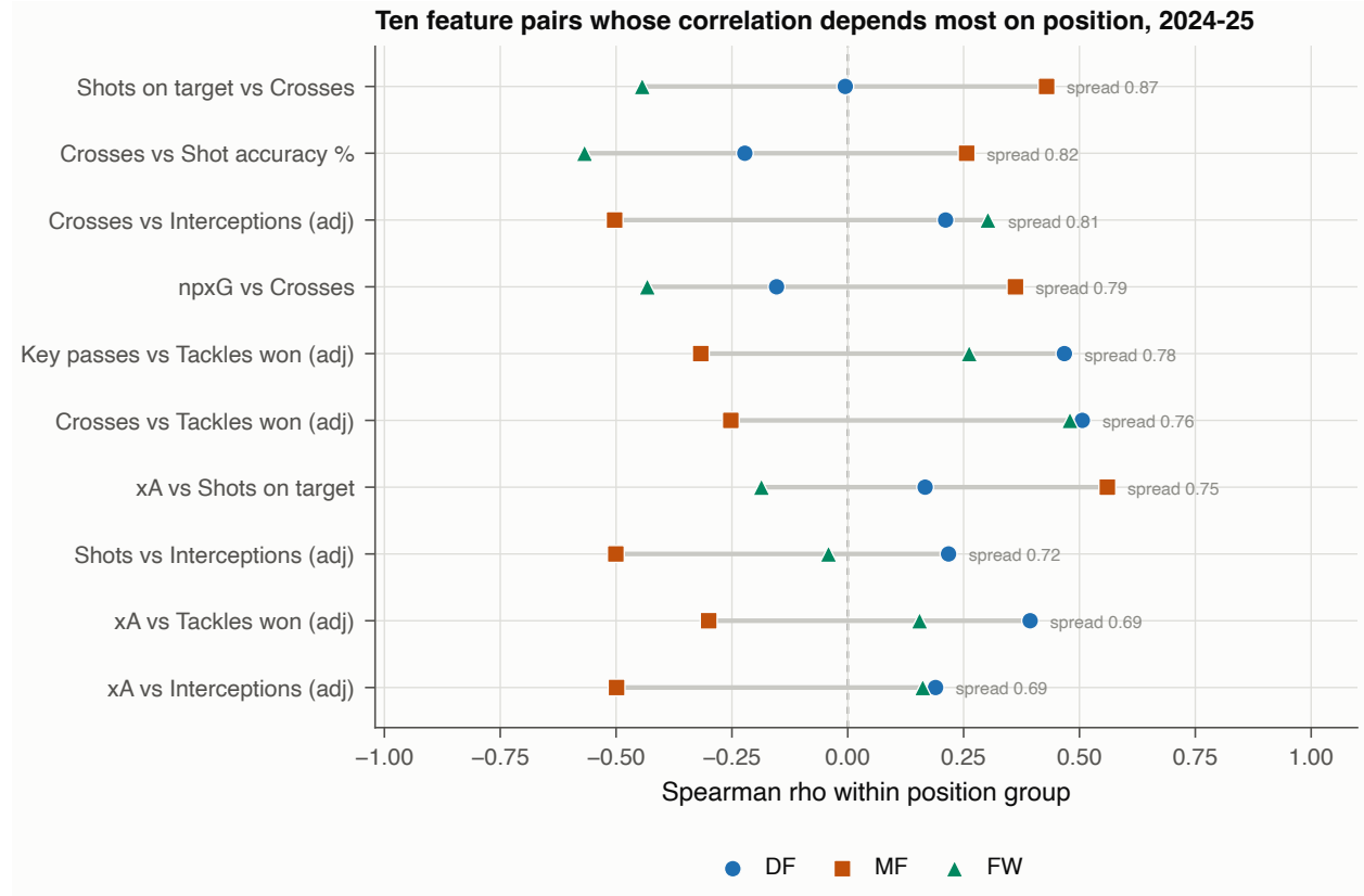
Figure 17: The ten feature pairs whose within-group correlation differs most across position groups in the earlier of the two reduced-sample seasons. Every pair changes sign between at least two groups.
