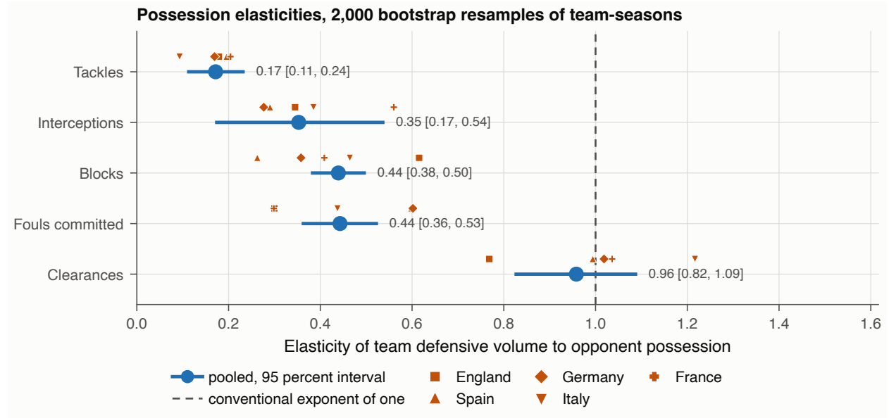
Figure 13: The five defensive possession elasticities with bootstrap intervals from 2,000 resamples of 490 team-seasons, against the conventional value of one, with each league's own refit shown as a smaller marker. Four intervals exclude one; the interval for clearances does not, and three league refits for clearances sit above one.
