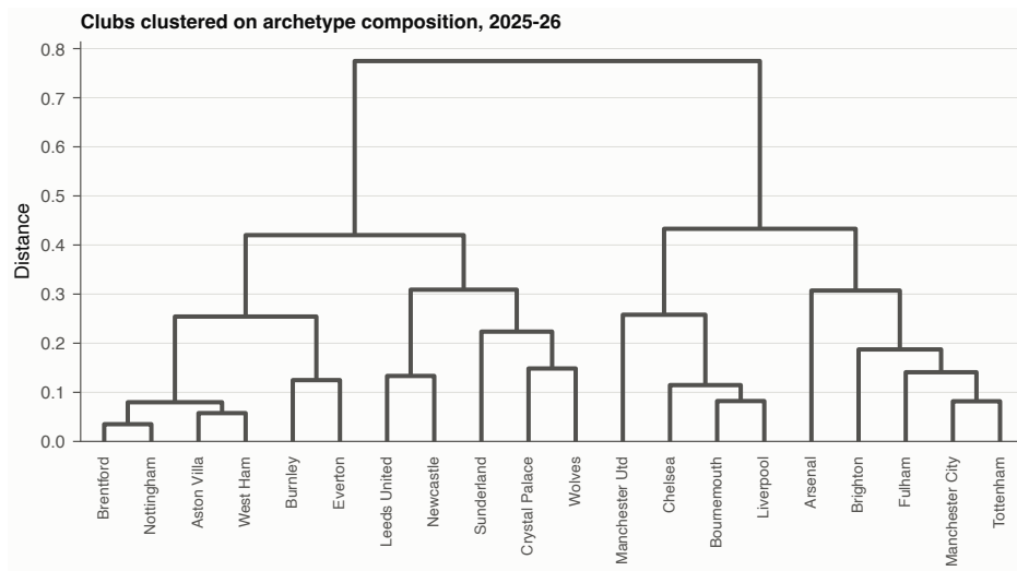
(a) Style families.
