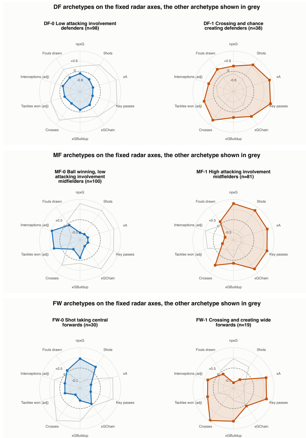
Figure 49: Archetype radars on the reduced sample.
