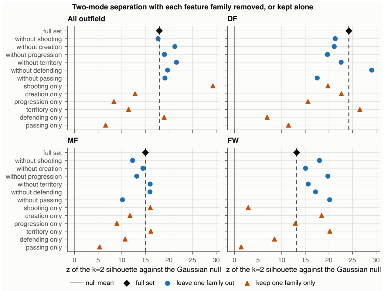
Figure 8: Standard score of the observed two-cluster silhouette against the clusterless null under every feature-family ablation, one panel per scope. Circles remove one family, triangles keep one family alone, and the vertical line is the full feature set. The adjusted Rand index against the full partition, which distinguishes the same two modes from a different pair, is in Table 3 and the text.
