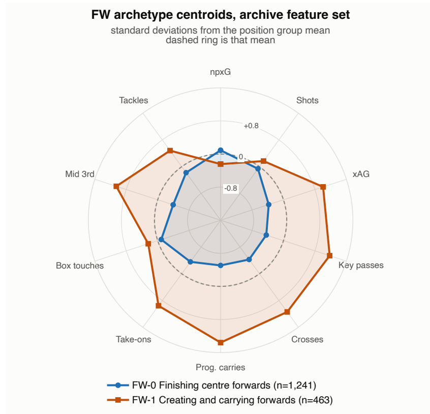
Figure 25: Forward archetypes, archive sample.
