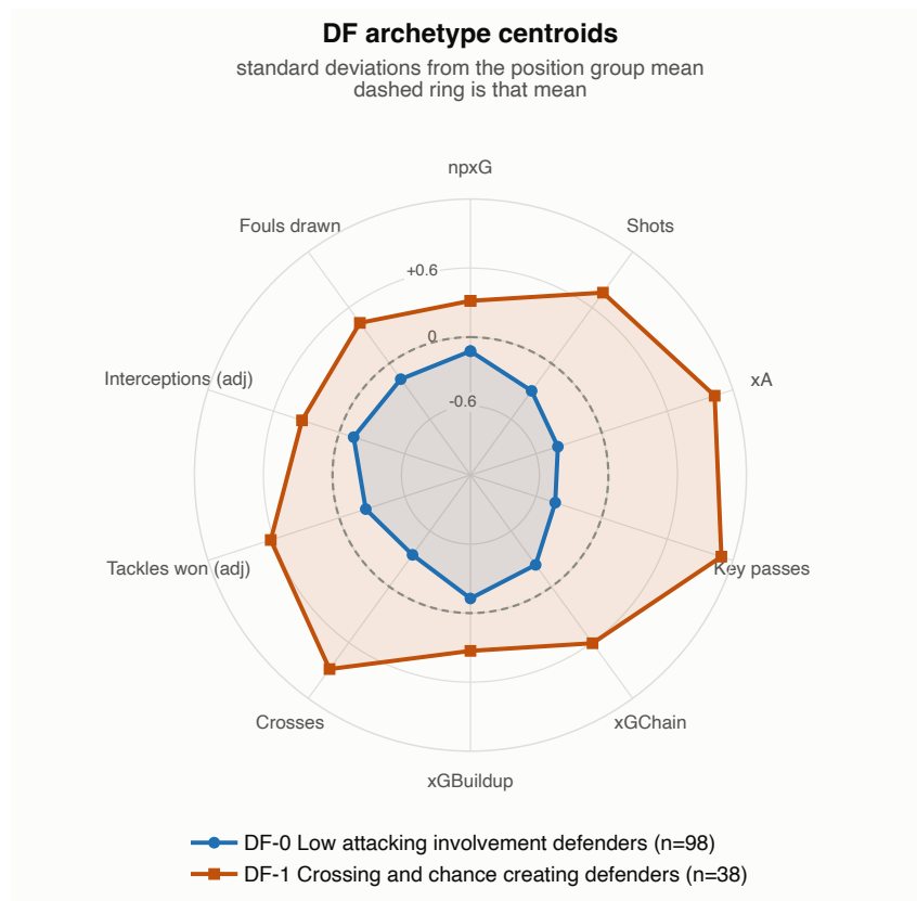
Figure 28: Defender archetypes.
