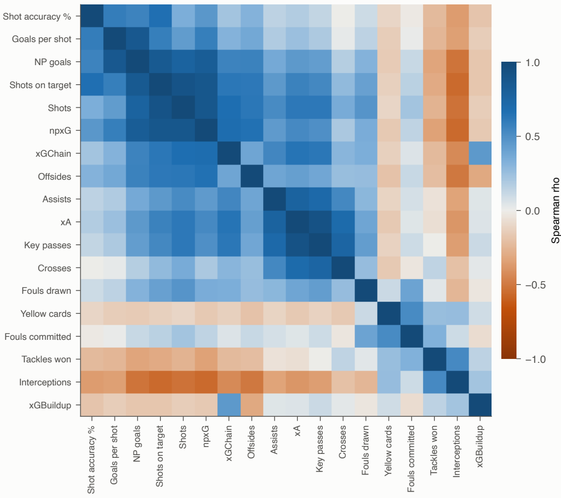
Spearman correlation, 18 surviving features, 2024-25 average-linkage ordering
